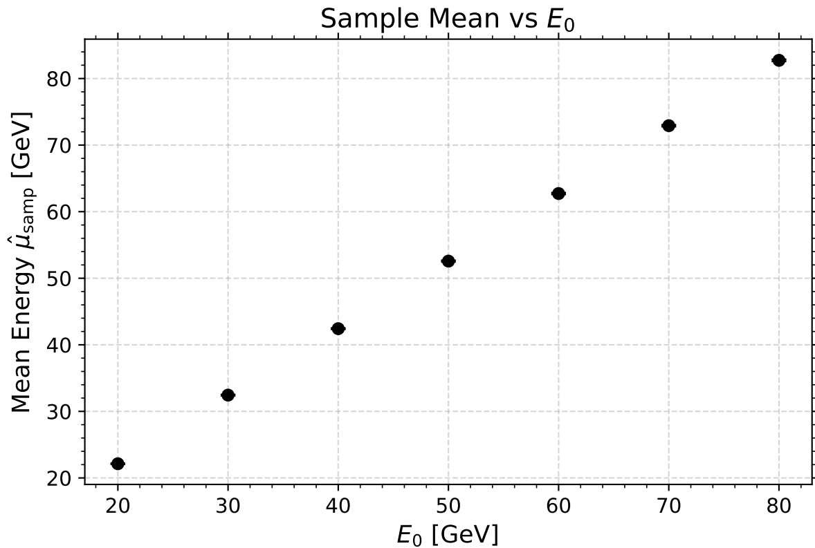
Figure 1.3: Sample Estimates
