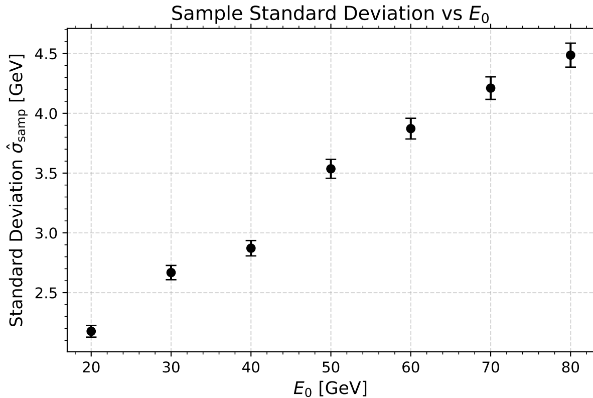
Figure 1.3: Sample Estimates
