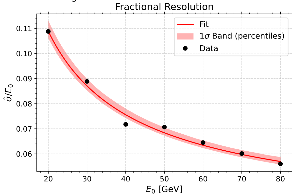
Figure 2.2: Individual MLE Fitting
