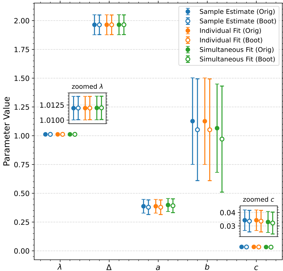
Fig 4.2: Comparison: Analytical vs Bootstrap Errors
