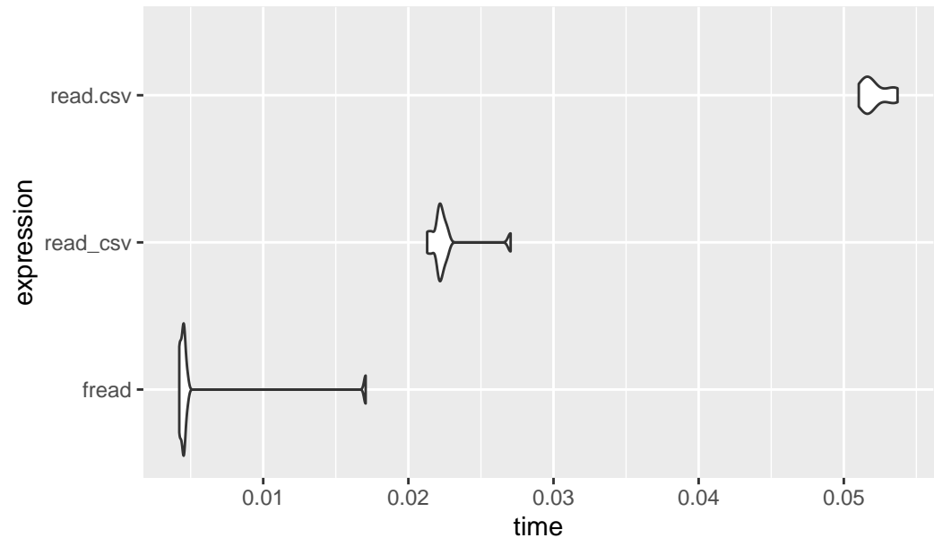
Time to read long-format file (selected columns)
