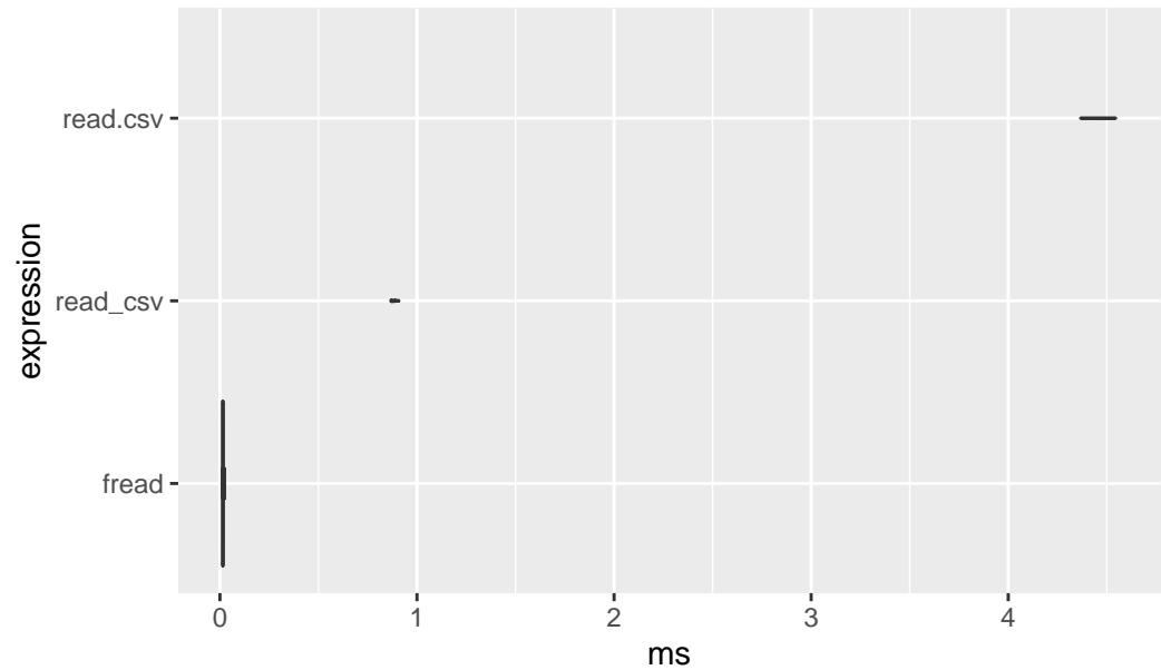
Time to read wide-format file
