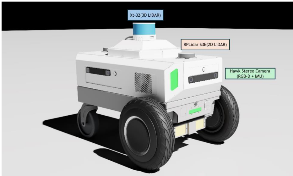
<Figure 7. Nova Carter>
