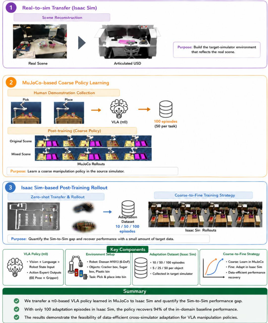
<Figure 2. Coarse-to-Fine Sim2Sim Adaptation Pipeline>
