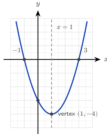
Figure 4.3 y = x^2 - 2x - 3 , with its vertex, axis of symmetry and intercepts.
