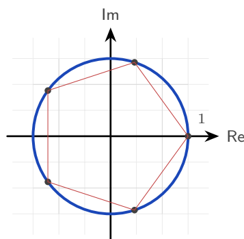
Figure 18.5 The five fifth roots of unity, at the vertices of a regular pentagon inscribed in the unit circle with one vertex at 1.
