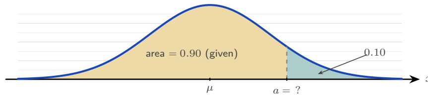
Figure 13.5 The inverse normal reverses the usual question. Instead of being given a and finding the area, you are given the area and must find a . A calculator expects the area to the left of a (gold), so a question phrased as a right-hand tail (teal), here 0.10, must be turned into its left-hand partner 0.90 first.
