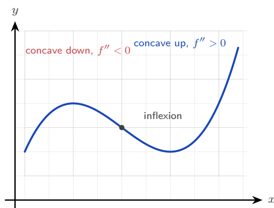
Figure 14.5 The second derivative decides which way the curve bends. Where the bending changes direction the curve has a point of inflexion.
