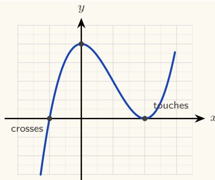
Figure 7.1 A sketch of y = (x + 1)(x - 2)^2 . The simple root at x = -1 crosses the axis; the double root at x = 2 touches it and turns back. The y -intercept is (0, 4) , and the ends follow x^3 .
