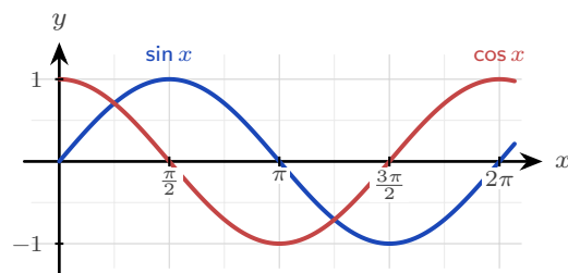
Figure 9.4 One turn of the circle unrolled. Both waves have amplitude 1 and period 2\pi ; the cosine is the sine shifted left by \frac{\pi}{2} .
