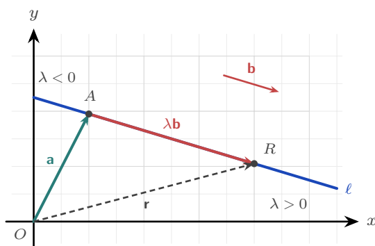
Figure 10.3 A line built from a point and a direction. The vector \mathbf{a} reaches the known point A ; travelling \lambda \mathbf{b} from there lands on a general point R , whose position vector \mathbf{r} closes the triangle. Negative \lambda runs back the other way, so the whole line is covered. The direction \mathbf{b} has no fixed home, so the free copy drawn above is the same vector.
