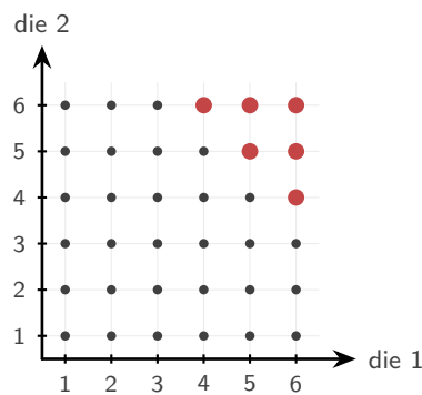
Figure 12.3 The 36 equally likely outcomes of rolling two dice. The six larger scarlet points are the outcomes whose total is at least 10.
