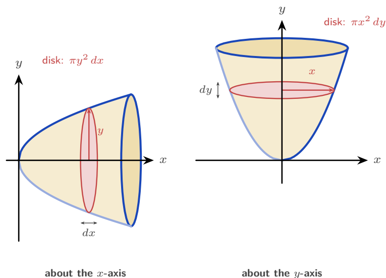
Figure 16.5 The same curve rotated about each axis. Turning it about the x -axis gives disks stacked along x : each has radius y and thickness dx , so its volume is \pi y^2 dx . Turning it about the y -axis gives disks stacked along y : each has radius x and thickness dy , so its volume is \pi x^2 dy . In both cases the integral adds the disks from one end of the solid to the other.
