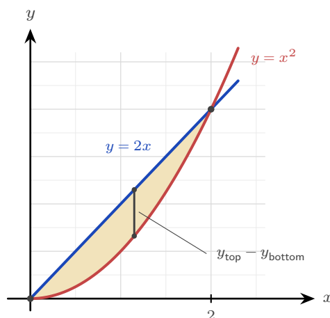
Figure 16.4 The region enclosed between y = 2x and y = x^2 . The curves meet where 2x = x^2 , at x = 0 and x = 2 , and the line is the upper boundary in between, so the area is \int_0^2 (2x - x^2) \, dx .
