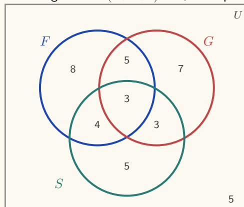
Figure 12.2 The three-circle diagram, filled from the centre outwards. The seven inner counts total
