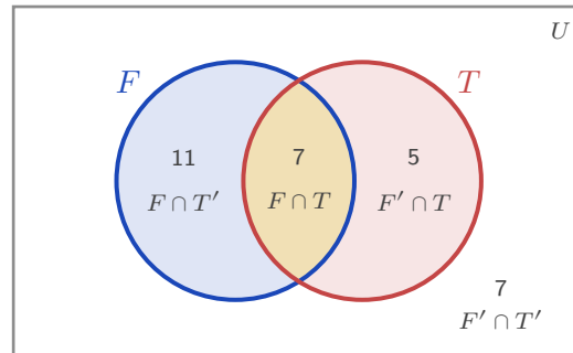
Figure 12.1 The four regions of a two-event Venn diagram, with the class of 30 filled in. Football only is F \cap T' , both is F \cap T , tennis only is F' \cap T , and neither is F' \cap T' , the region outside both circles. The four counts add to 30.
