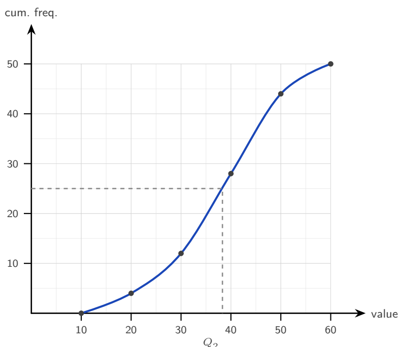
Figure 11.2 A cumulative frequency curve for 50 values. Each point is plotted at the upper boundary of its class. The dashed line reads the median: enter at half the total frequency, cross to the curve, drop to the value axis.
