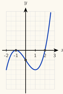
Figure 7.2 The curve touches the x -axis at x = -1 , crosses it at x = 2 , and passes through (0, -1) . These three facts determine the equation.
