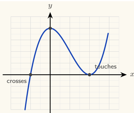
Figure 7.1 A sketch of y = (x + 1)(x - 2)^2 . The simple root at x = -1 crosses the axis; the double root at x = 2 touches it and turns back. The y -intercept is (0, 4) , and the ends follow x^3 . Every factorised polynomial is sketched the same way: the roots and their multiplicities give the behaviour at the x -axis, the value at x = 0 gives the y -intercept, and the leading term gives the two ends.
