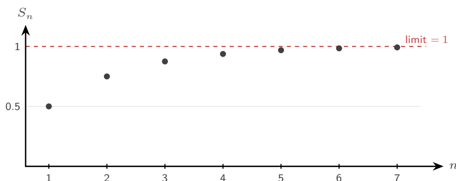
Figure 2.3 The partial sums of \frac{1}{2} + \frac{1}{4} + \frac{1}{8} + \dots climb toward 1 but never pass it.
