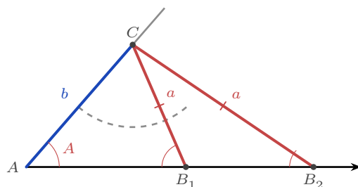
Figure 8.3 Two sides and a non-included angle. Swinging the fixed length a from C meets the base at B_1 and at B_2 , so two different triangles have the same a, b and A . The angles at B_1 and B_2 add to 180^\circ , which is why the sine rule returns both.
