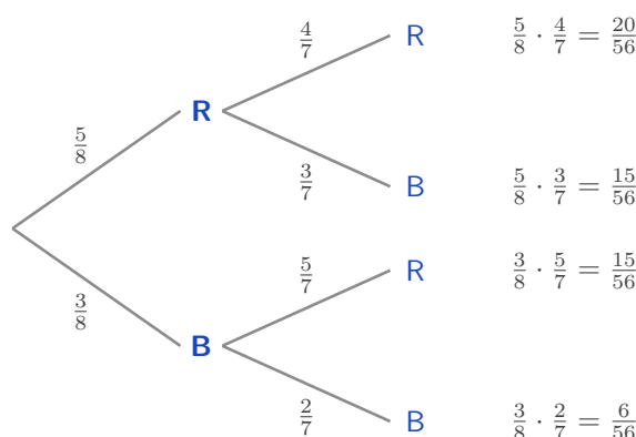
Figure 12.4 A tree diagram for drawing two marbles from 5 red and 3 blue without replacement. The probabilities on the second stage differ from the first, because one marble has already been removed.
