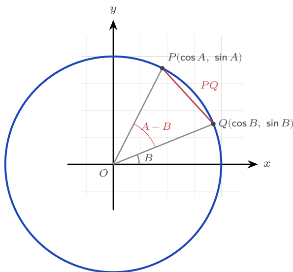
Figure 9.3 Two points on the unit circle, at angles A and B . The angle between the radii is A - B , and the chord PQ can be measured either by the distance formula or by the cosine rule.
