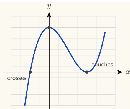
Figure 7.1 A sketch of y = (x + 1)(x - 2)^2 . The simple root at x = -1 crosses the axis; the double root at x = 2 touches it and turns back. The y -intercept is (0, 4) , and the ends follow x^3 . Every factorised polynomial is sketched the same way: the roots and their multiplicities give the behaviour at the x -axis, the value at x = 0 gives the y -intercept, and the leading term gives the two ends.
