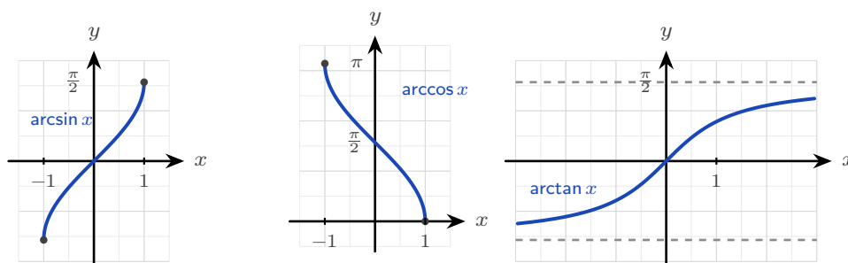
Figure 9.7 Each inverse is its restricted parent reflected in y = x . The marked endpoints show the range
