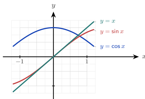
Figure 14.1 Near the origin the graphs of \sin x and x are almost the same, so their ratio tends to 1. But \cos x tends to 1 while x tends to 0, so \frac{\cos x}{x} has no finite limit.
