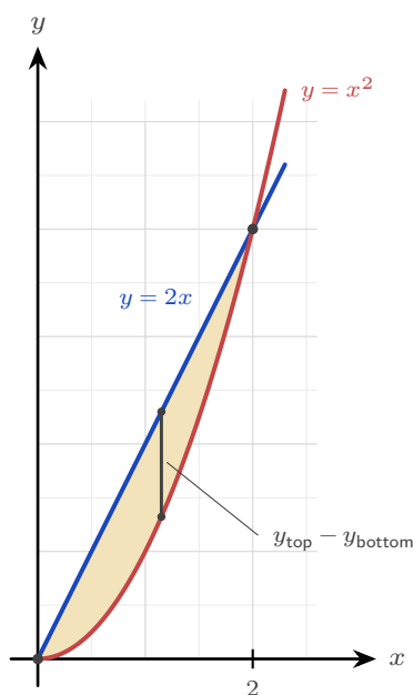
Figure 16.4 The region enclosed between y = 2x and y = x^2 . The curves meet where 2x = x^2 , at x = 0 and x = 2 , and the line is the upper boundary in between, so the area is \int_0^2 (2x - x^2) dx .
