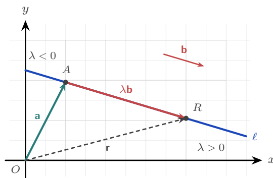
Figure 10.3 A line built from a point and a direction. The vector \mathbf{a} reaches the known point A ; travelling \lambda\mathbf{b} from there lands on a general point R , whose position vector \mathbf{r} closes the triangle. Negative \lambda runs back the other way, so the whole line is covered. The direction \mathbf{b} has no fixed home, so the free copy drawn above is the same vector.
