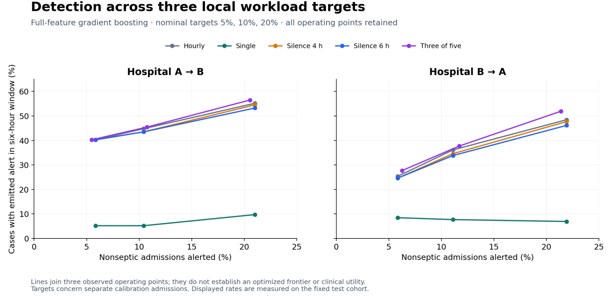
Figure 3: Exploratory observed admission false-alert rate versus six-hour any-emission sensitivity at nominal local targets of 5%, 10% and 20%, full-feature boosting. Lines connect the three evaluated targets; they are not fitted optimal frontiers. Each rule is calibrated separately on the same held-out local calibration pool.
