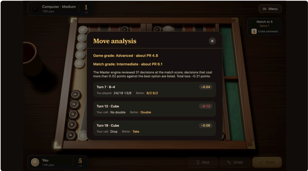
FIGURE 5.7 Move analysis.
