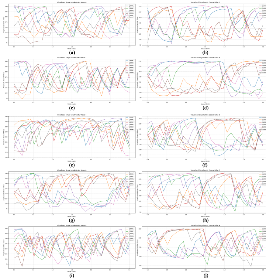
Gambar 3.2 Hasil Segmentasi Data dari Setiap Class Hand Gesture : (a) Hand Open , (b) Hand Close , (c) Fine Grip , (d) Pointer , (e) Agree , (f) Two , (g) Three , (h) Four , (i) Pinch , dan (j) Half Close .
