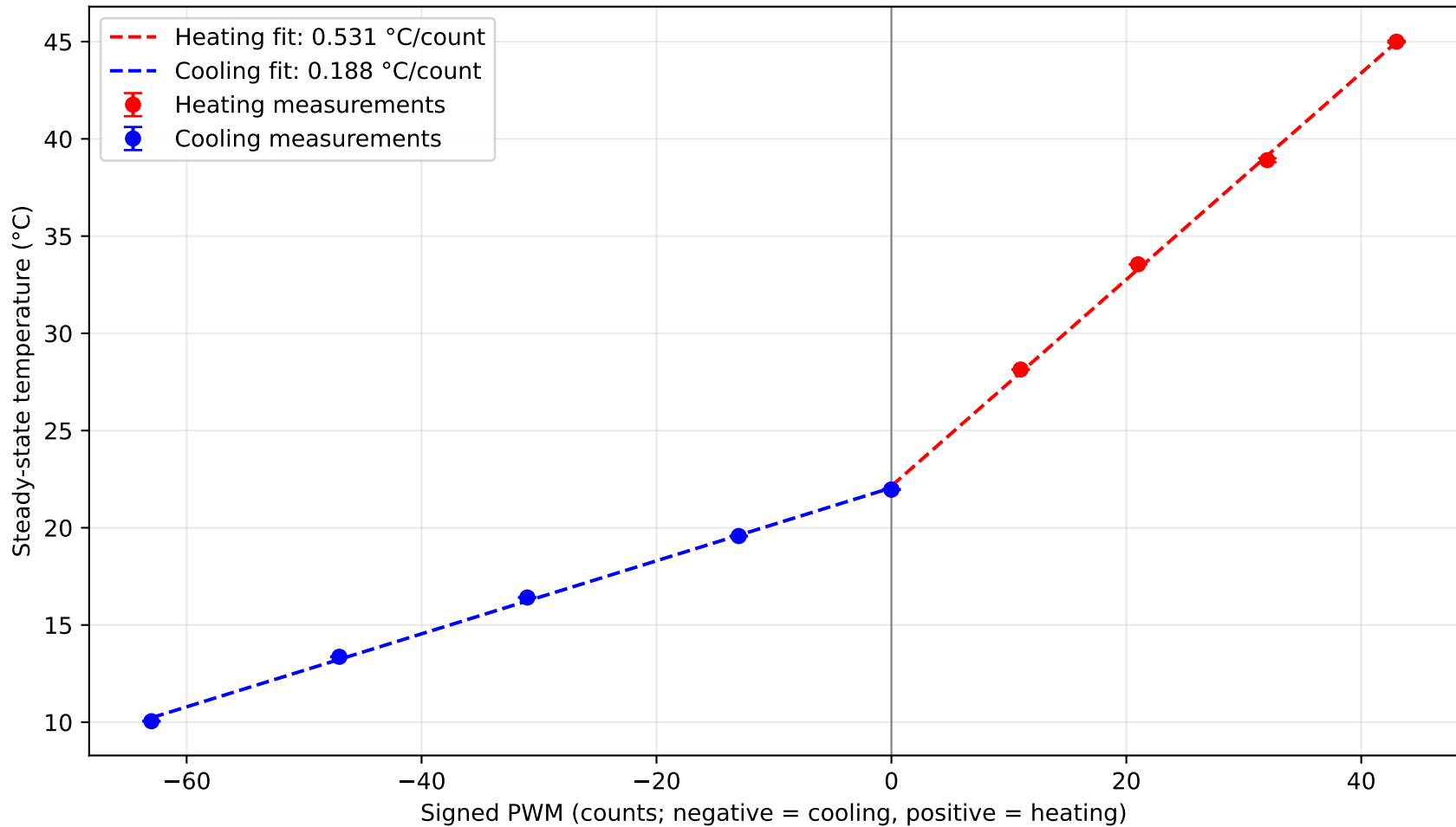
TEC steady-state temperature versus signed PWM
