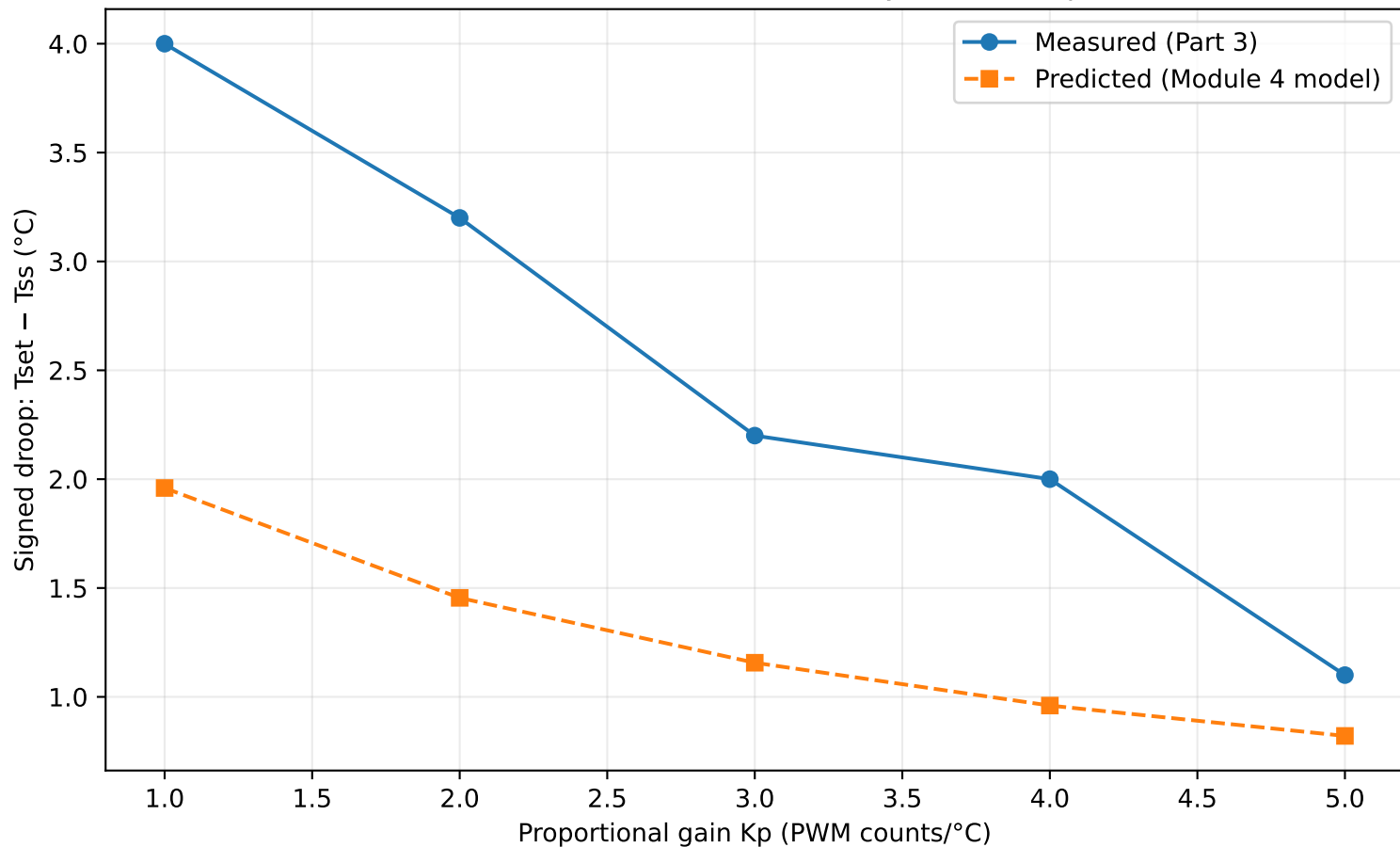
Predicted and measured steady-state droop
