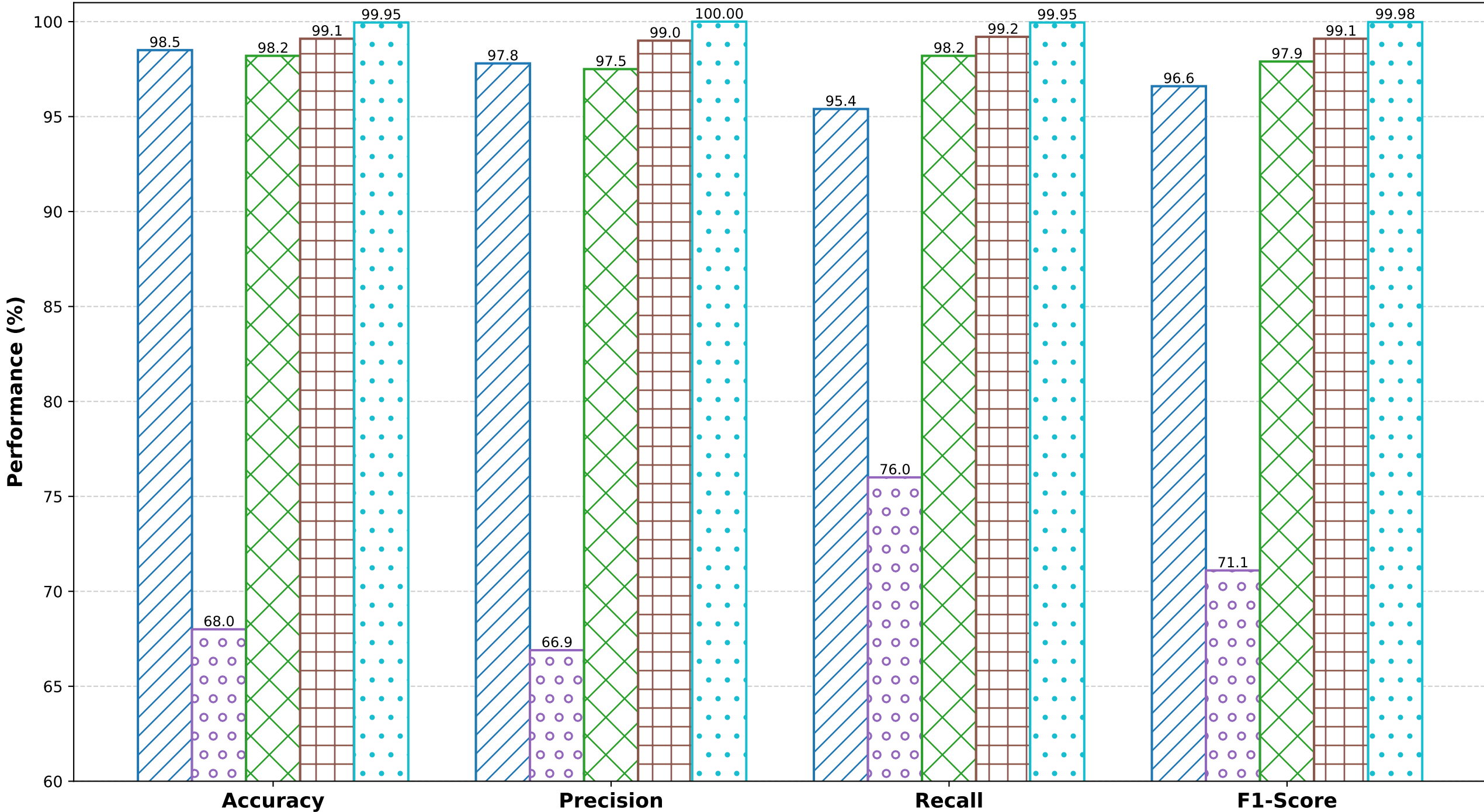
Comparison of Proposed Model with Existing Methods (Baseline 2)
