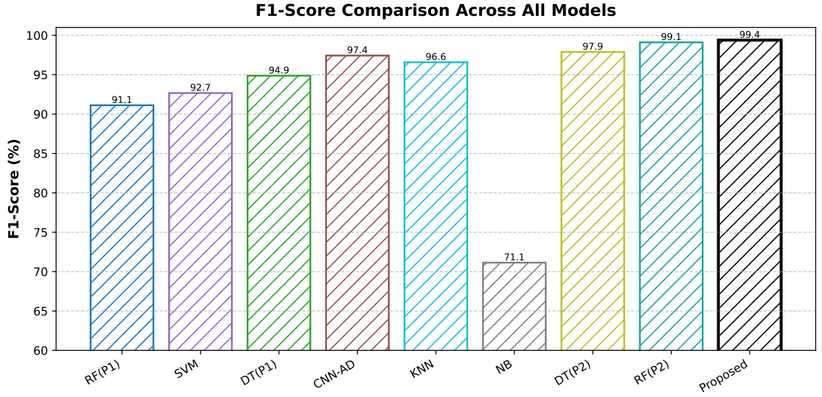
FIGURE 7 | F1-score comparison of the proposed CNN-LSTM model with machine learning and deep learning models reported in Baseline 1 [67] and Baseline 2 [68] on the CICDDoS2019 dataset.
