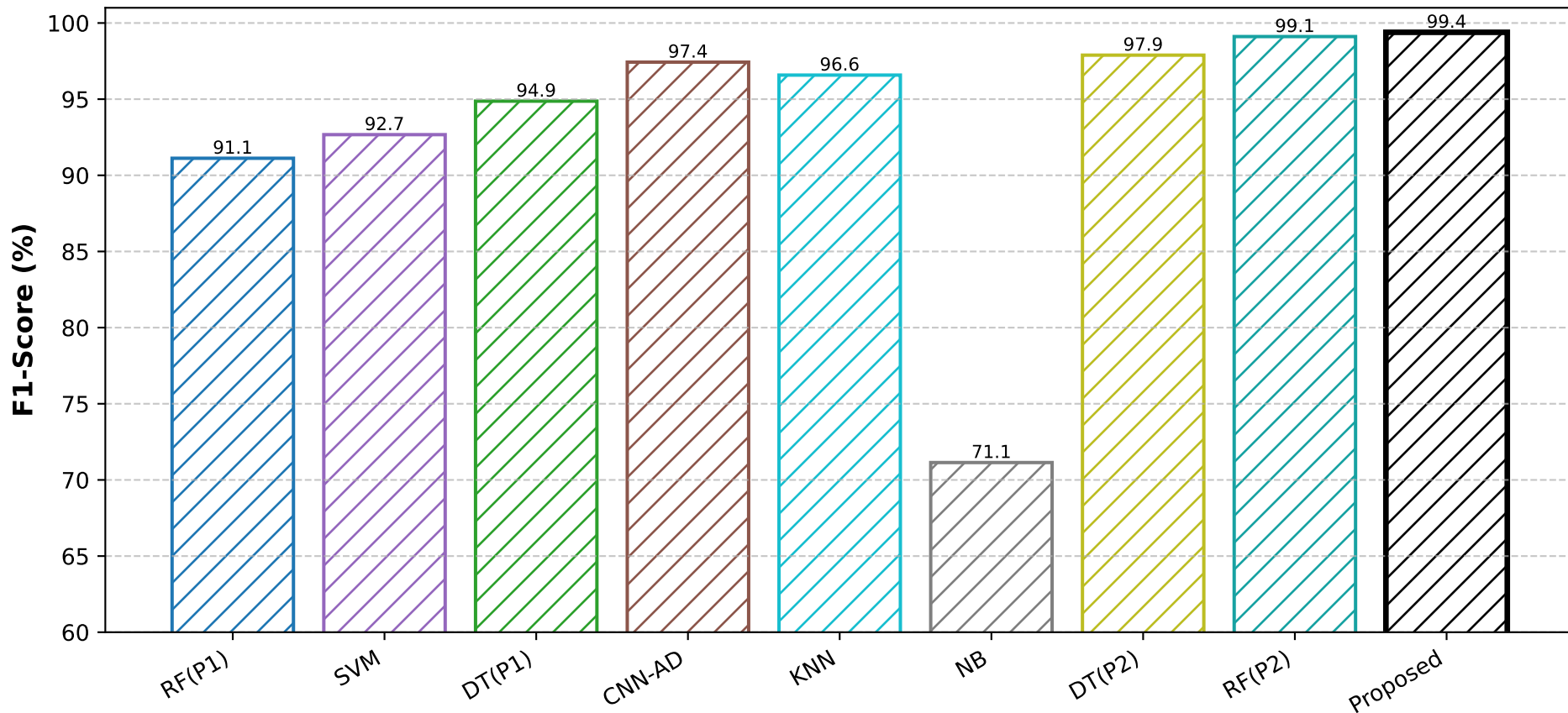
F1-Score Comparison Across All Models
