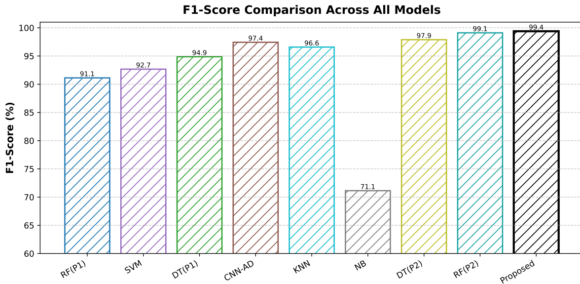
FIGURE 7 | F1-score comparison of the proposed CNN-LSTM model with machine learning and deep learning models reported in Baseline 1 [67] and Baseline 2 [66] on the CICDDoS2019 dataset.
