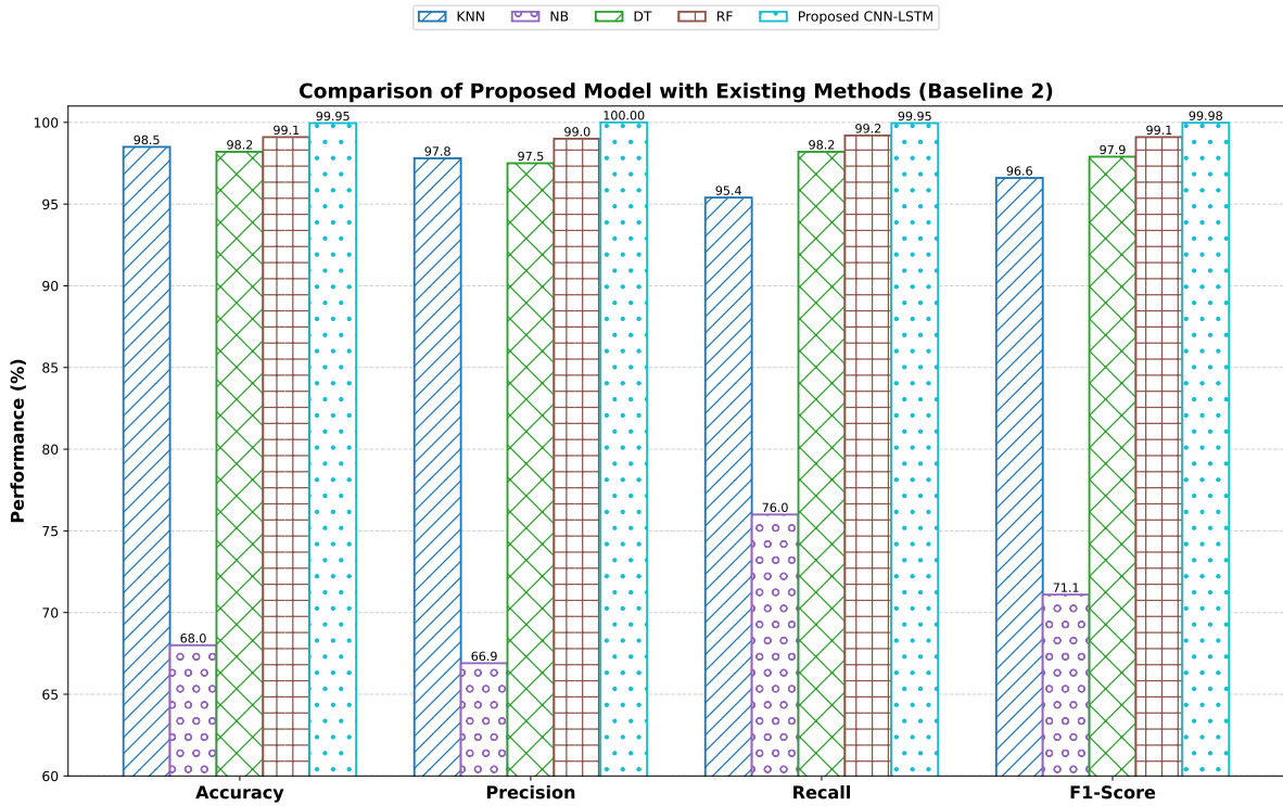
FIGURE 6 | Performance comparison of the proposed CNN-LSTM model with baseline machine learning and deep learning methods reported in [68] (Baseline 2) in terms of accuracy, precision, recall, and F1-score on the CICDDoS2019 dataset.
