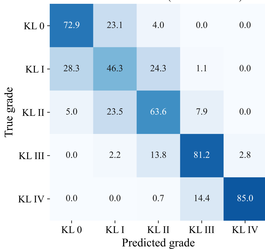
ProtoNet + Ordinal (DenseNet-121)
