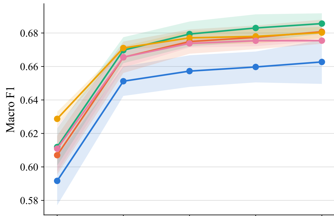
ResNet-18
