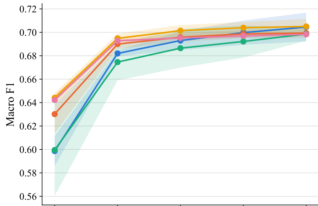
DenseNet-121
