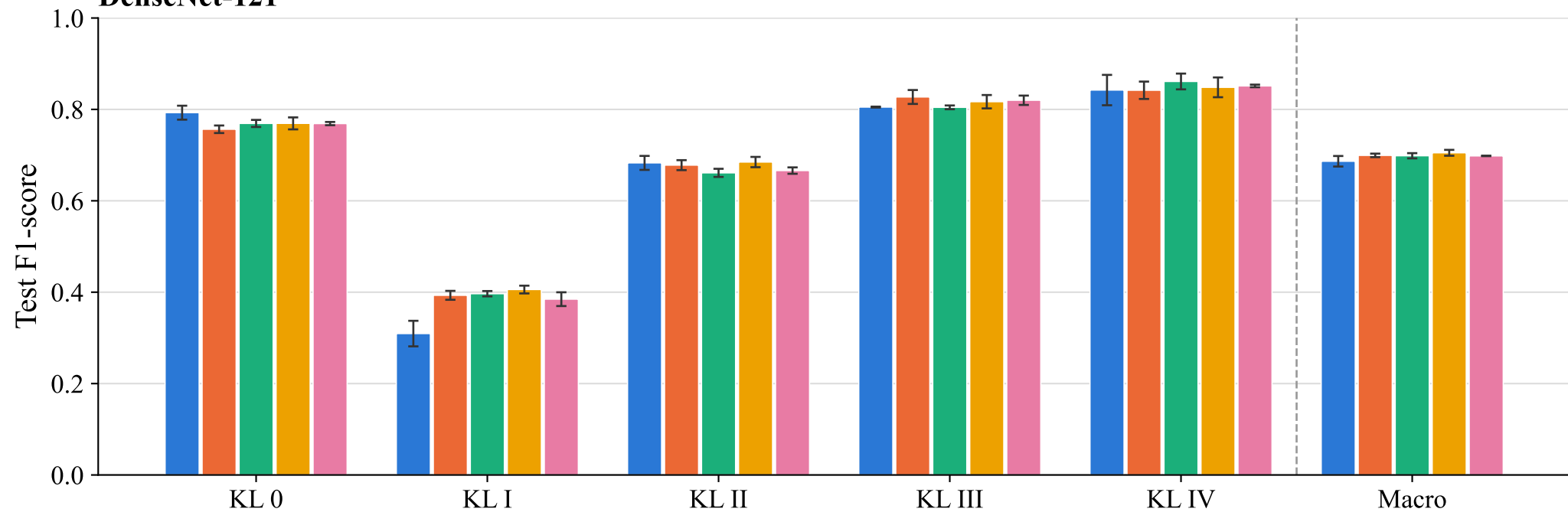
DenseNet-121
