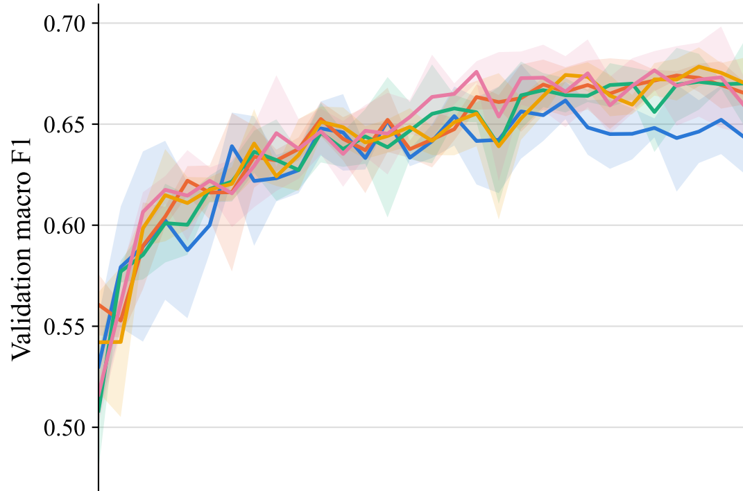
ResNet-18
