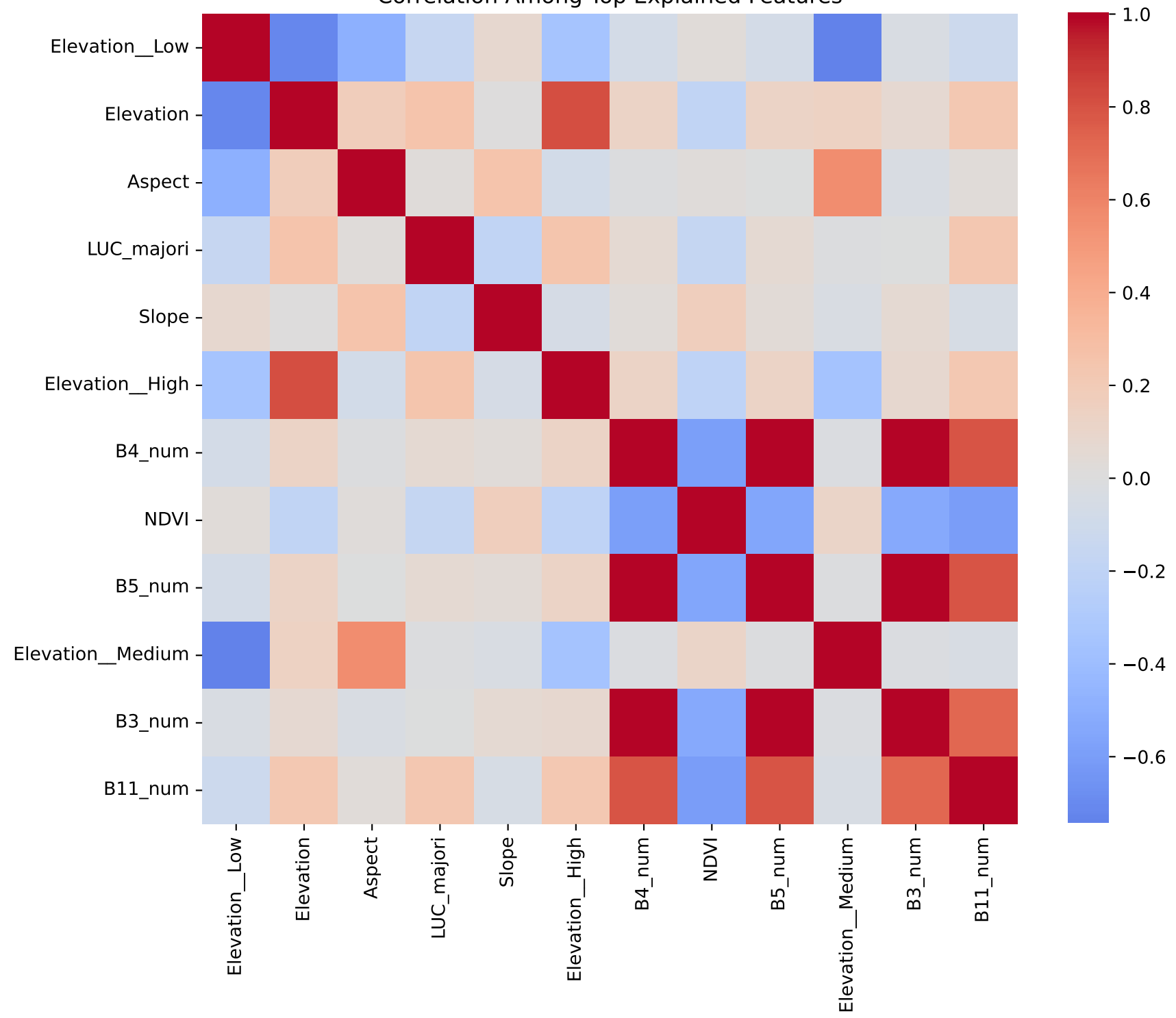
Correlation Among Top Explained Features
