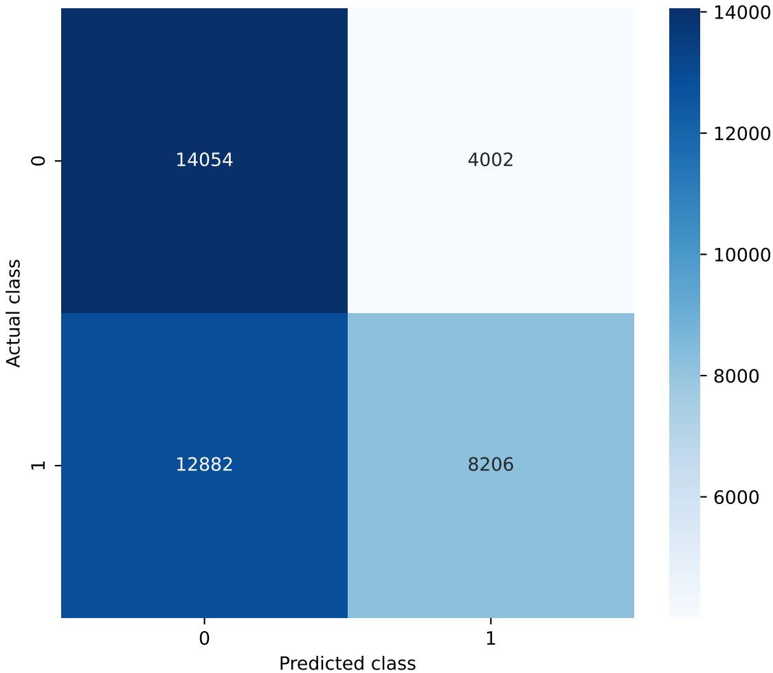
New Model Confusion Matrix
