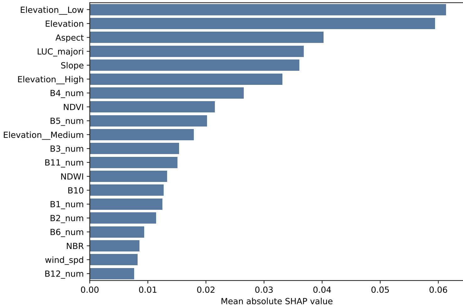
Top 20 SHAP Feature Importance
