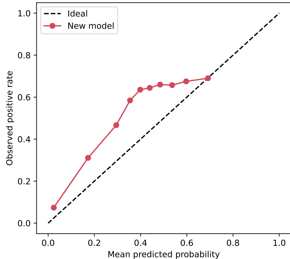
Probability Calibration
