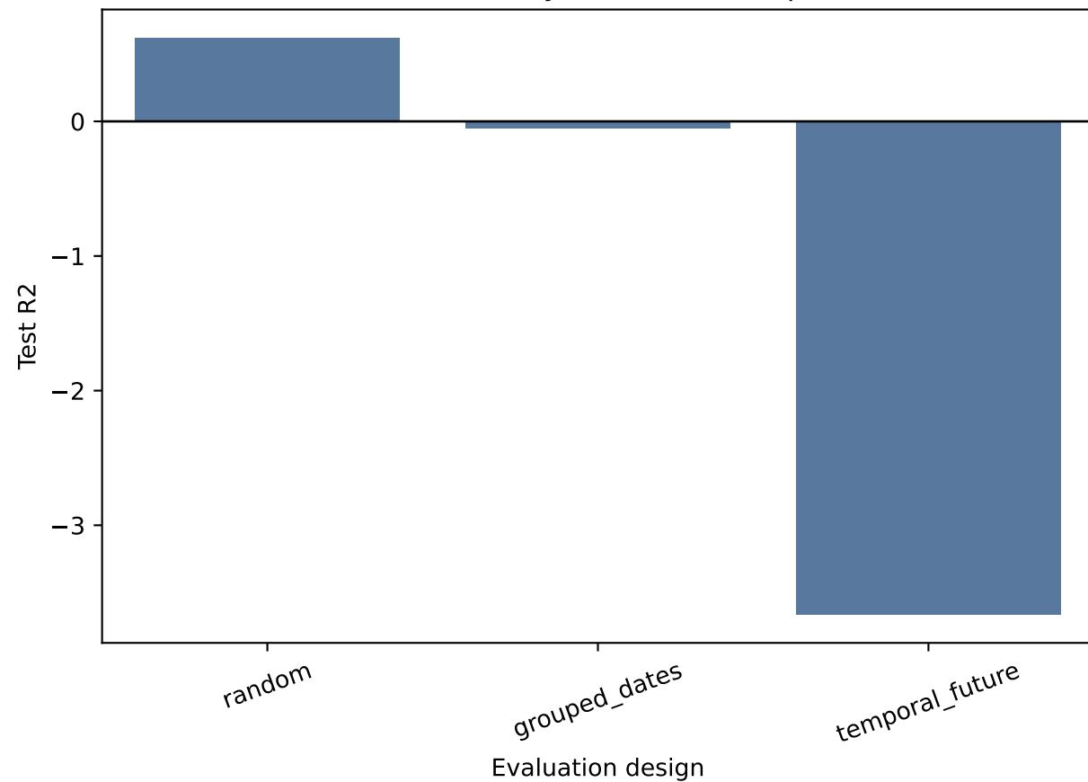
R2 Sensitivity to Evaluation Split
