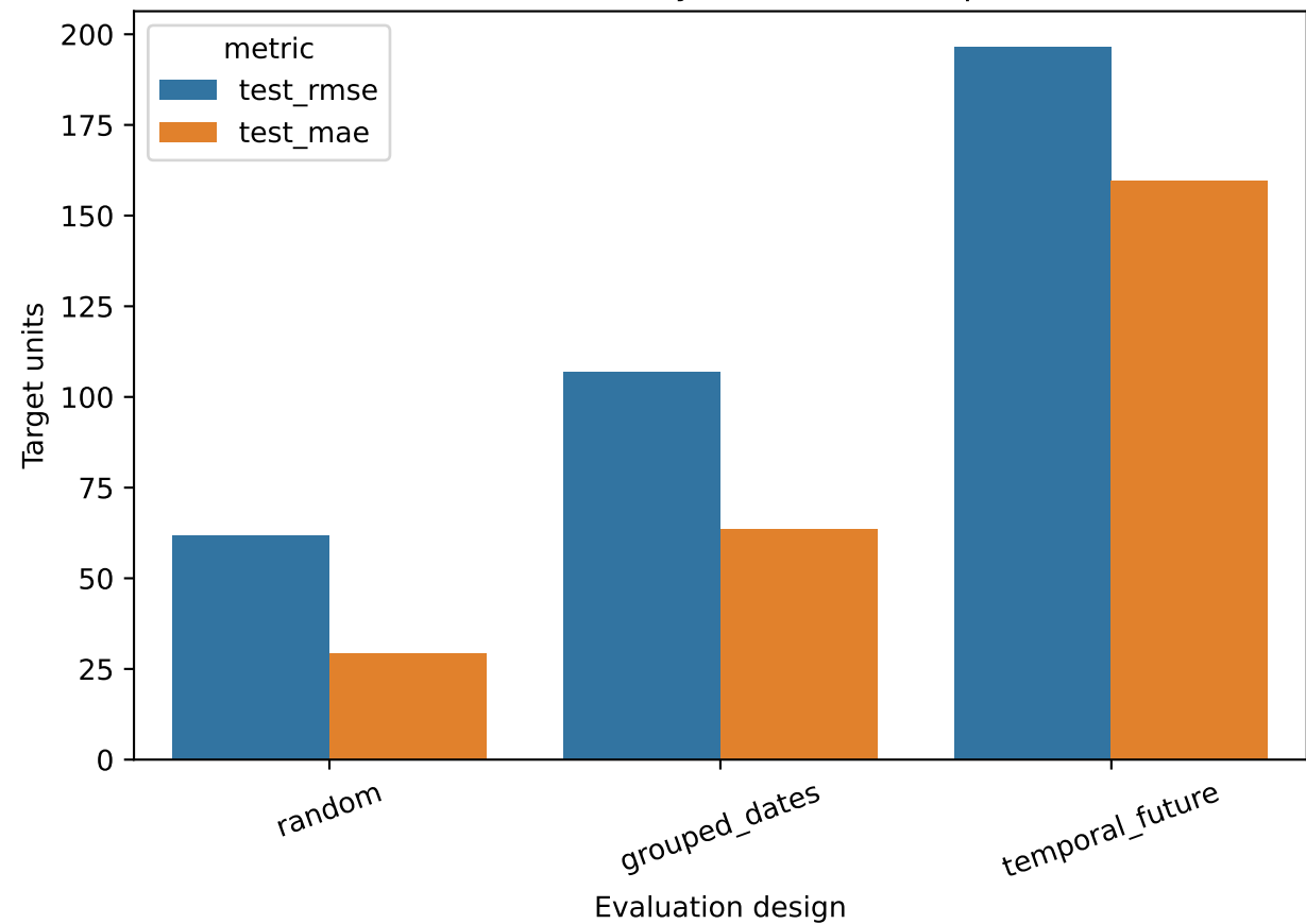
Error Sensitivity to Evaluation Split
