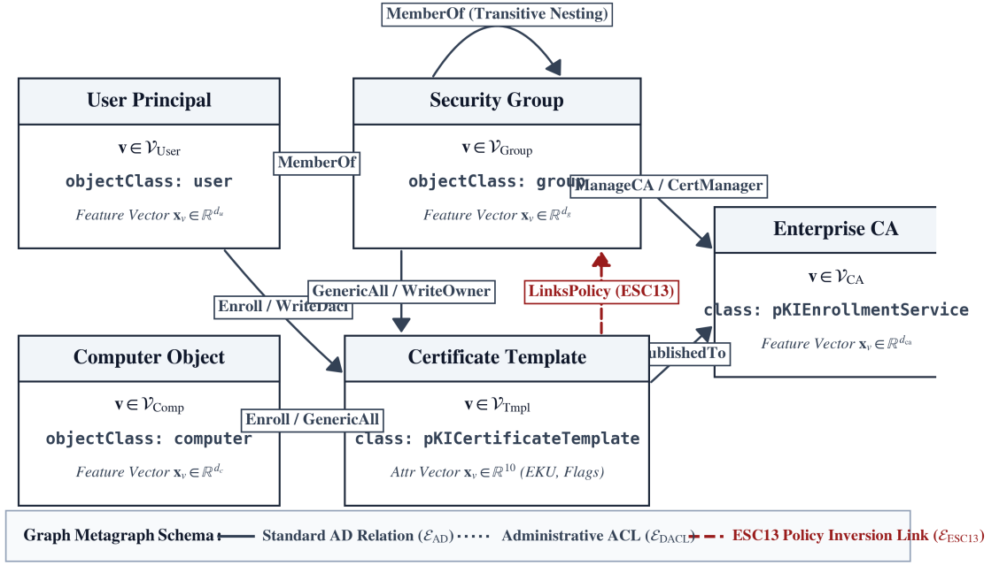
Figure 2.1: Heterogeneous Active Directory Certificate Services (ADCS) Graph Schema, illustrating relations between security principals (Users, Computers, Groups), Certificate Templates, and Enterprise Certificate Authorities.
