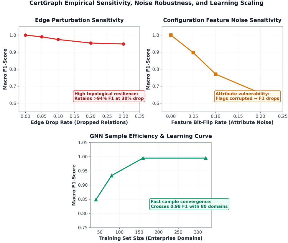
Figure 7.2: GNN robustness evaluation under systematic edge deletions (collection gaps), configuration feature noise (attribute corruption), and training data efficiency scaling.
