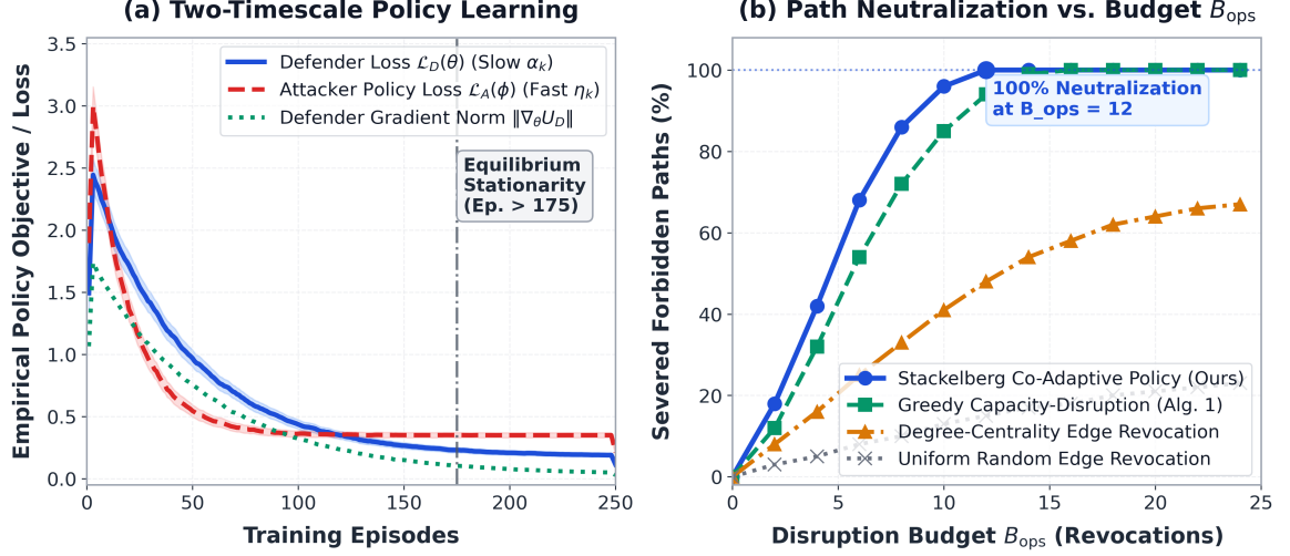
Figure 9.1: Autonomous cyber defense evaluation: (a) Notional two-timescale policy learning dynamics showing asymptotic decay of defender policy loss and gradient norm under the stochastic approximation framework. (b) Forbidden compromise path neutralization rate as a function of operational disruption budget B_{\text{ops}} , comparing measured empirical performance for Uniform Random, Degree-Centrality, and Greedy Capacity-Disruption (Alg. 4) across 30 Active Directory topologies against the notional trajectory of the co-adaptive Stackelberg model. Shaded bands denote \pm 1 standard deviation.
