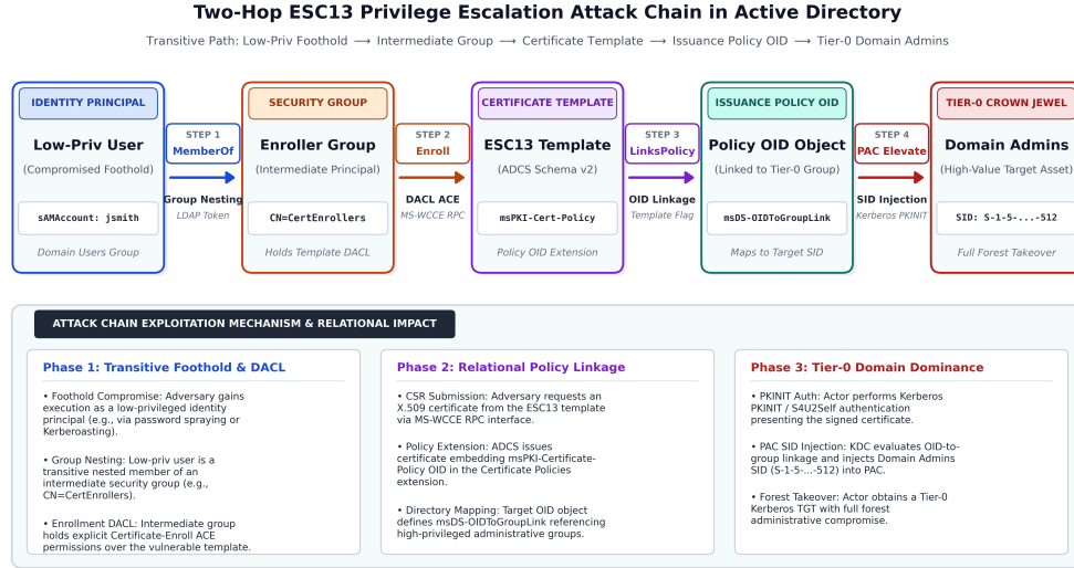
Figure 2: Two-hop ESC13 privilege escalation attack path, showing the chain from an unprivileged user through enrollment permissions and issuance policy OID linkage to high-value domain administrative group tokens.
