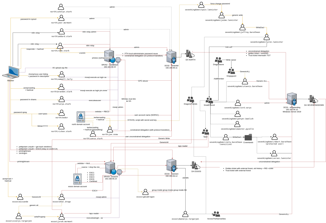
Figure 10: End-to-end multi-hop compromise and privilege escalation attack graph across the GOAD domain infrastructure, illustrating how unprivileged foothold credentials traverse AD CS certificate misconfigurations (ESC1–ESC8), Kerberos delegations, and inter-domain trusts to achieve enterprise domain dominance.
