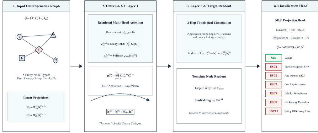
Figure 3: CertGraph end-to-end Hetero-GAT pipeline, detailing input feature encoding, multi-head relational attention layers, additive residual skip-connections, and the multi-class template classification head.
