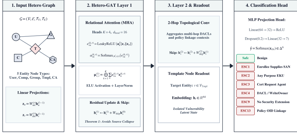
Figure 3: CertGraph end-to-end Hetero-GAT pipeline, detailing input feature encoding, multi-head relational attention layers, additive residual skip-connections, and the multi-class template classification head.
