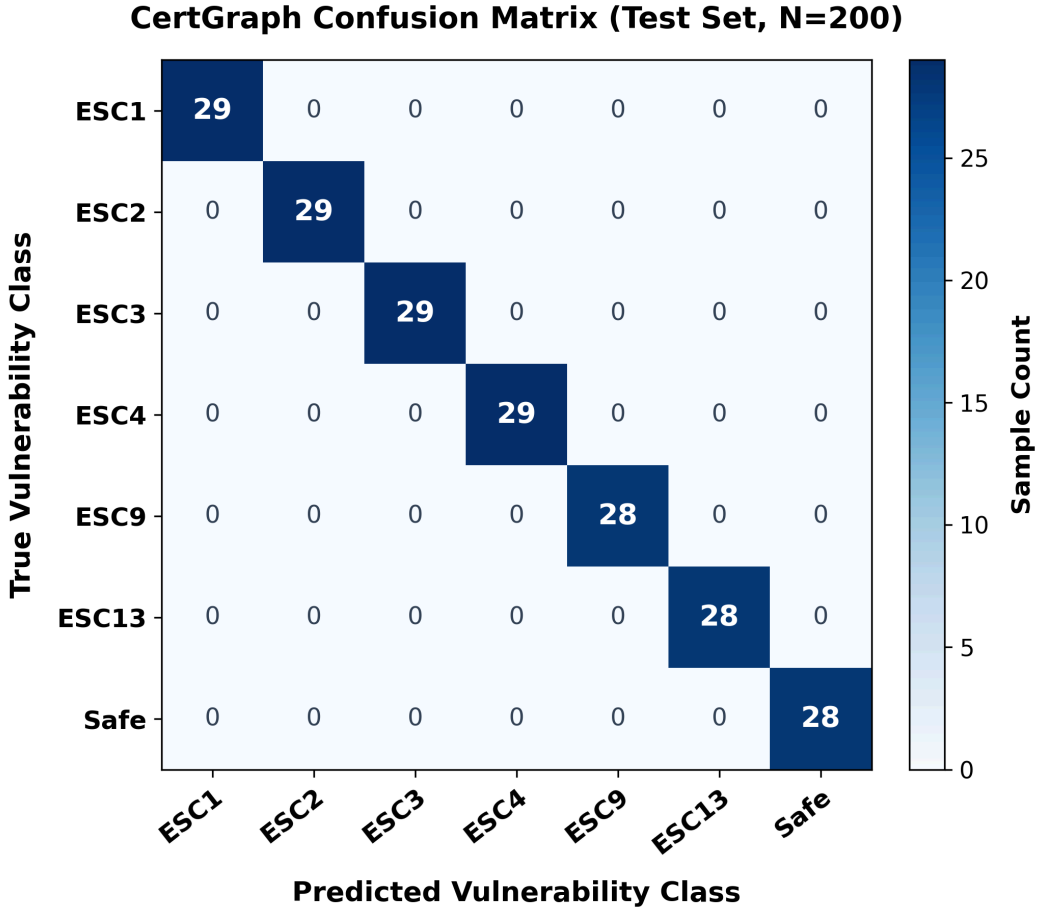
Figure 5: CertGraph 7-Class Confusion Matrix.
