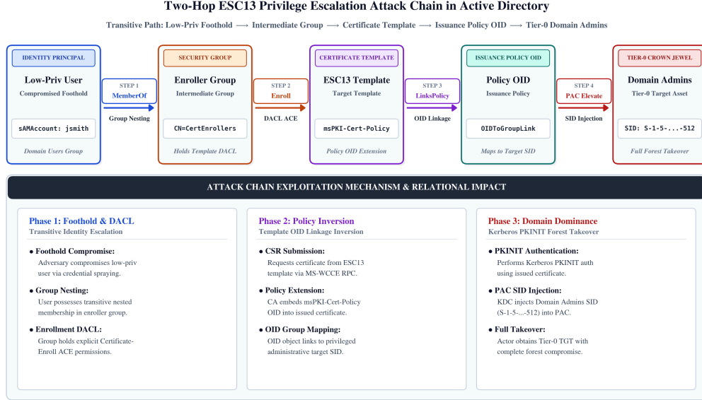
Figure 2: Two-hop ESC13 privilege escalation attack path, showing the chain from an unprivileged user through enrollment permissions and issuance policy OID linkage to high-value domain administrative group tokens.
