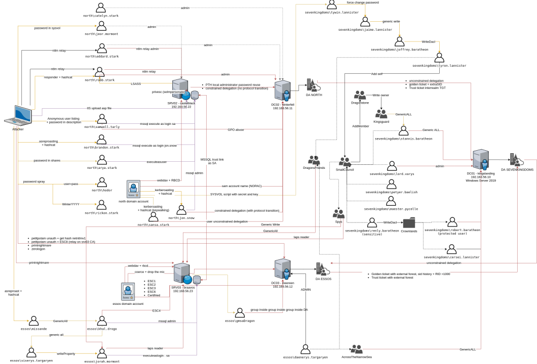
Figure 10: End-to-end multi-hop compromise and privilege escalation attack graph across the GOAD domain infrastructure, illustrating how unprivileged foothold credentials traverse ADCS certificate misconfigurations (ESC1–ESC8), Kerberos delegations, and inter-domain trusts to achieve enterprise domain dominance.
