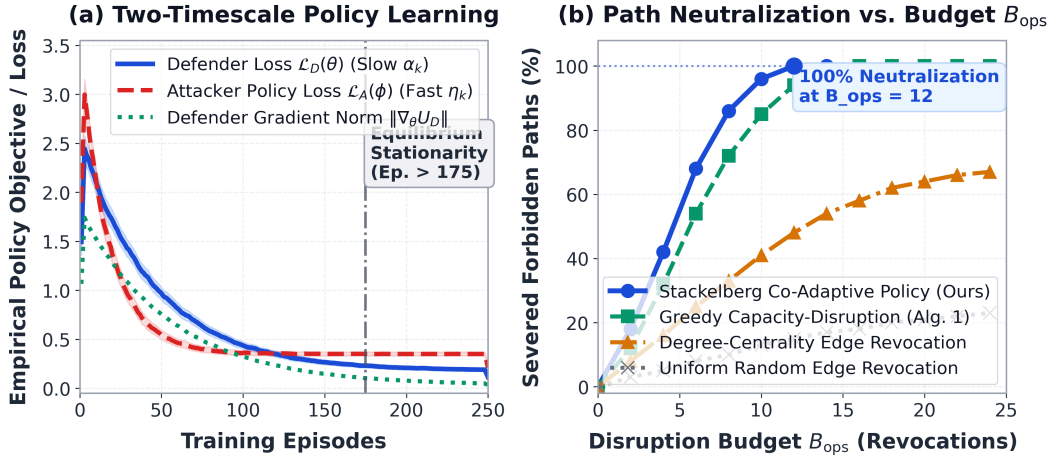
Figure 15: Autonomous cyber defense evaluation: (a) Notional two-timescale policy learning dynamics showing asymptotic decay of defender policy loss and gradient norm under the stochastic approximation framework. (b) Forbidden compromise path neutralization rate as a function of operational disruption budget B_{\text{ops}} , comparing measured empirical performance for Uniform Random, Degree-Centrality, and Greedy Capacity-Disruption (Alg. Algorithm 4) across 30 Active Directory topologies against the notional trajectory of the co-adaptive Stackelberg model. Shaded bands denote \pm 1 standard deviation.
