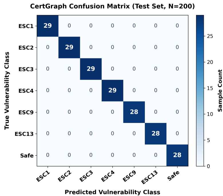
(a) CertGraph 7-Class Confusion Matrix.
