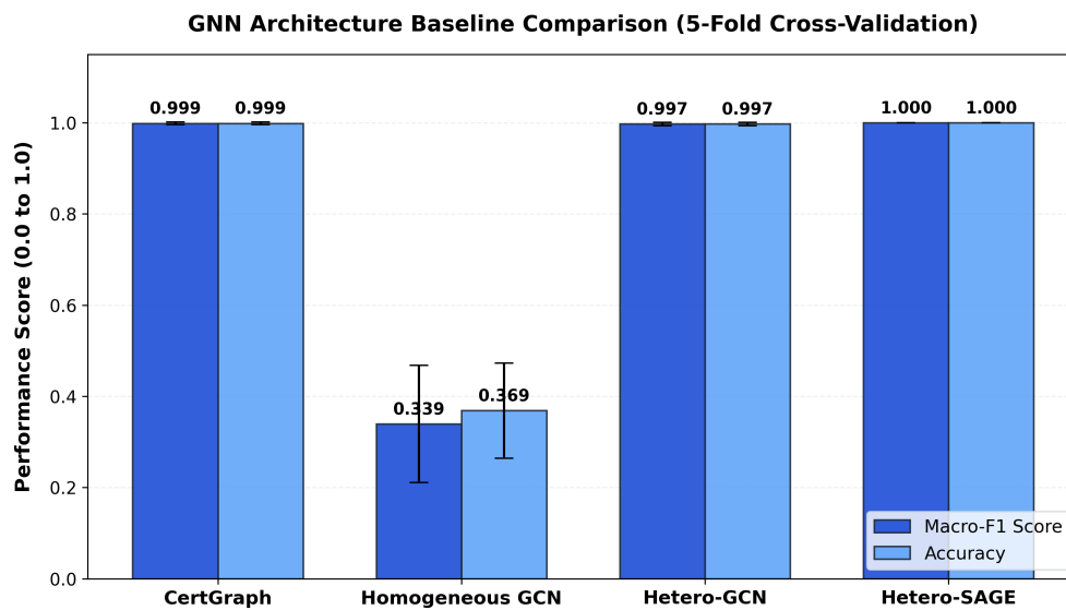
(b) GNN Family Comparison.
