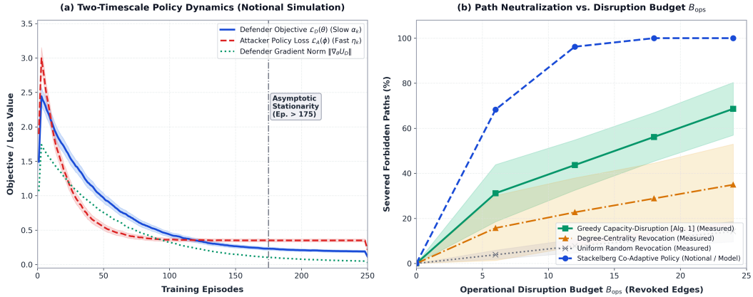
Figure 15: Autonomous cyber defense evaluation: (a) Notional two-timescale policy learning dynamics showing asymptotic decay of defender policy loss and gradient norm under the stochastic approximation framework. (b) Forbidden compromise path neutralization rate as a function of operational disruption budget B_{\text{ops}} , comparing measured empirical performance for Uniform Random, Degree-Centrality, and Greedy Capacity-Disruption (Alg. Algorithm 4) across 30 Active Directory topologies against the notional trajectory of the co-adaptive Stackelberg model. Shaded bands denote \pm 1 standard deviation.
