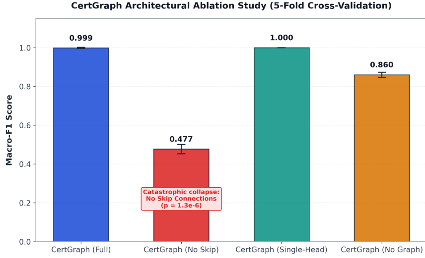
Figure 5.2: Ablation study comparison highlighting the performance collapse when residual skip connections are disabled.
