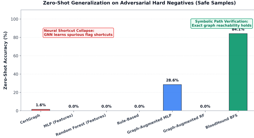
Figure 5.3: Zero-shot adversarial evaluation demonstrating the collapse of pure neural models due to shortcut learning compared to symbolic BFS path traversal.
