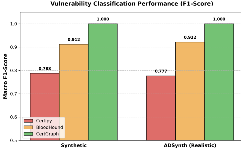
Figure 7.1: Comparative performance (CertGraph vs BloodHound vs Certiply) across synthetic and ADSynth realistic tiered enterprise topologies.
