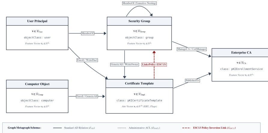
Figure 2.1: Heterogeneous Active Directory Certificate Services (ADCS) Graph Schema, illustrating relations between security principals (Users, Computers, Groups), Certificate Templates, and Enterprise Certificate Authorities.
