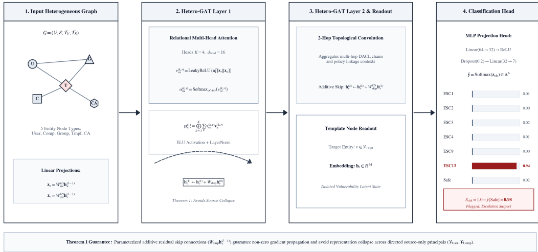
Figure 3.1: CertGraph end-to-end Hetero-GAT pipeline, detailing input feature encoding, multi-head relational attention layers, additive residual skip-connections, and the multi-class template classification head.
