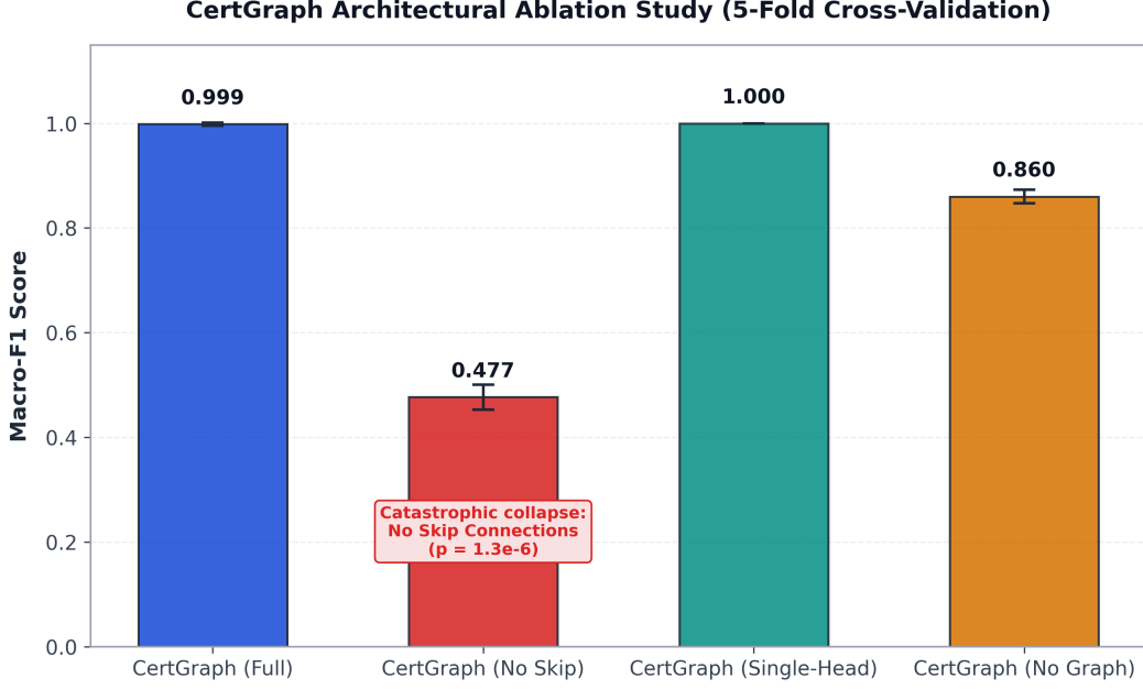
Figure 6: Ablation study comparison highlighting the performance collapse when residual skip connections are disabled.
