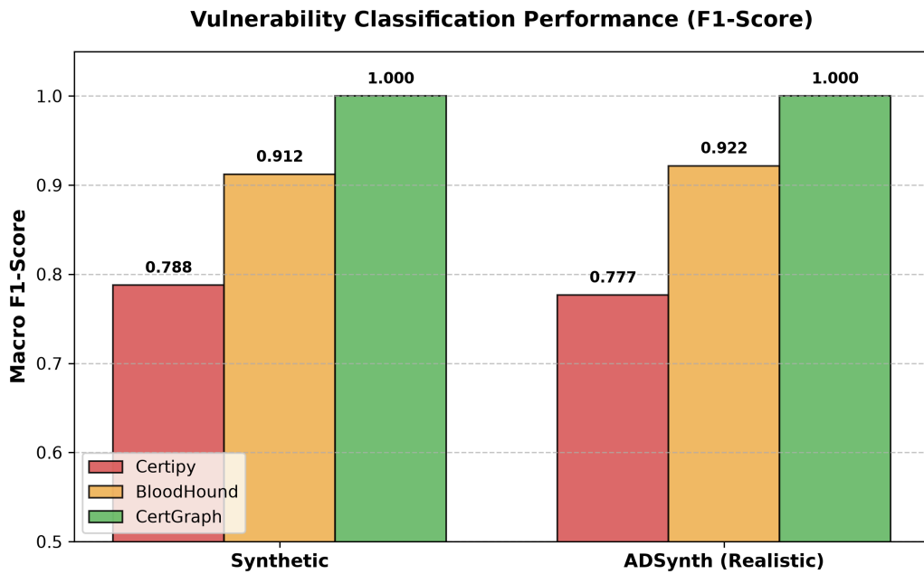
Figure 11: Comparative performance (CertGraph vs BloodHound vs Certipy) across synthetic and ADSynth realistic tiered enterprise topologies.
