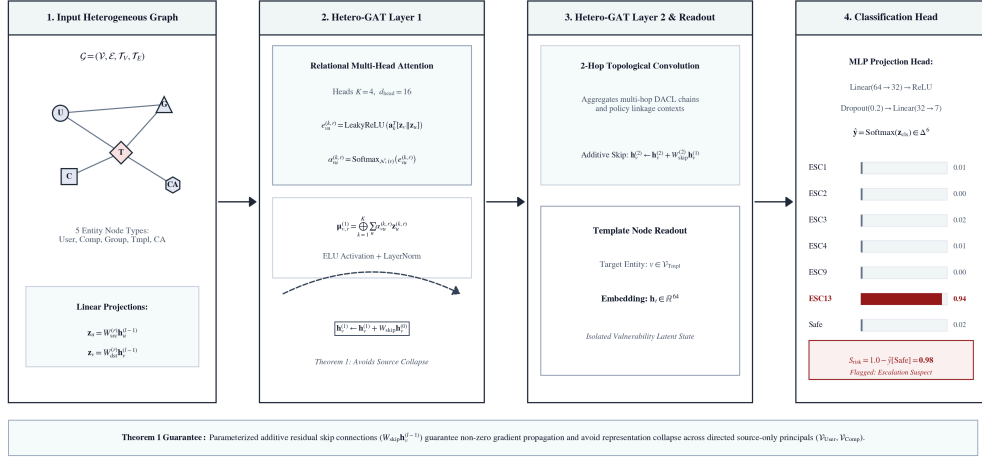
Figure 3: CertGraph end-to-end Hetero-GAT pipeline, detailing input feature encoding, multi-head relational attention layers, additive residual skip-connections, and the multi-class template classification head.
