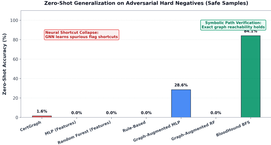
Figure 7: Zero-shot adversarial evaluation demonstrating the collapse of pure neural models due to shortcut learning compared to symbolic BFS path traversal.
