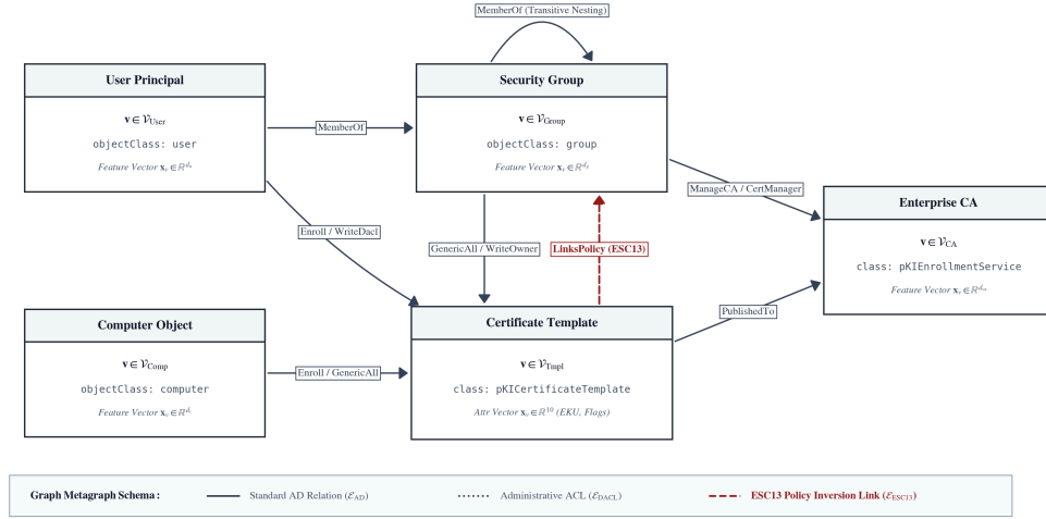
Figure 1: Heterogeneous Active Directory Certificate Services (ADCS) Graph Schema, illustrating relations between security principals (Users, Computers, Groups), Certificate Templates, and Enterprise Certificate Authorities.
