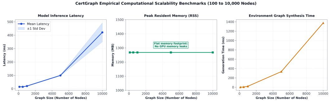
Figure 13: Scalability benchmarks showing empirical inference latency scaling sub-linearly with graph volume while Resident Set Size (RSS) process memory remains flat and bounded.
