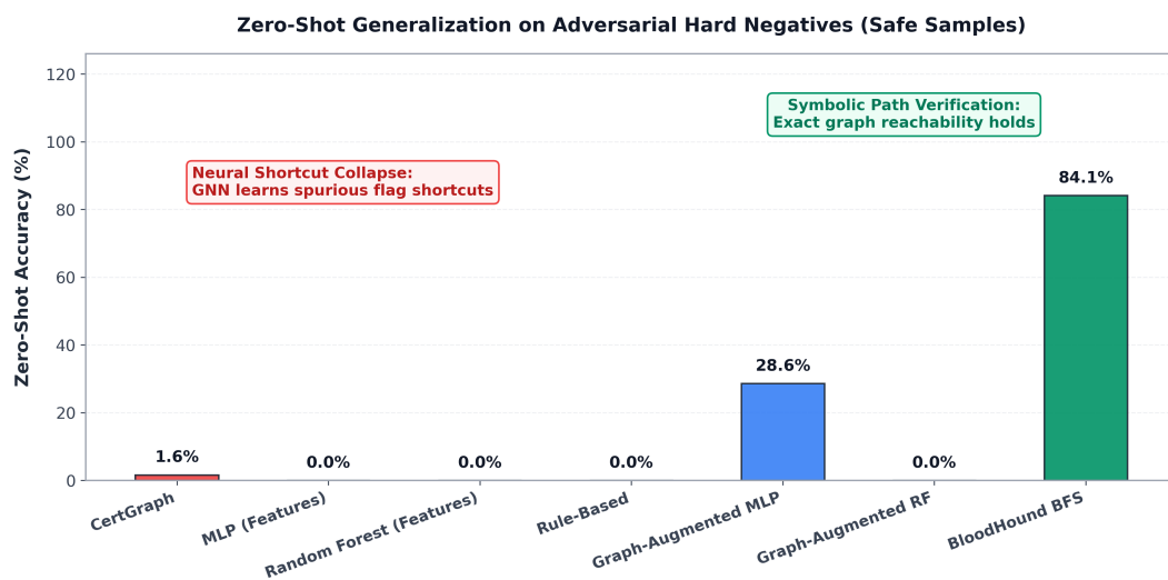
Figure 5.3: Zero-shot adversarial evaluation demonstrating the collapse of pure neural models due to shortcut learning compared to symbolic BFS path traversal.
