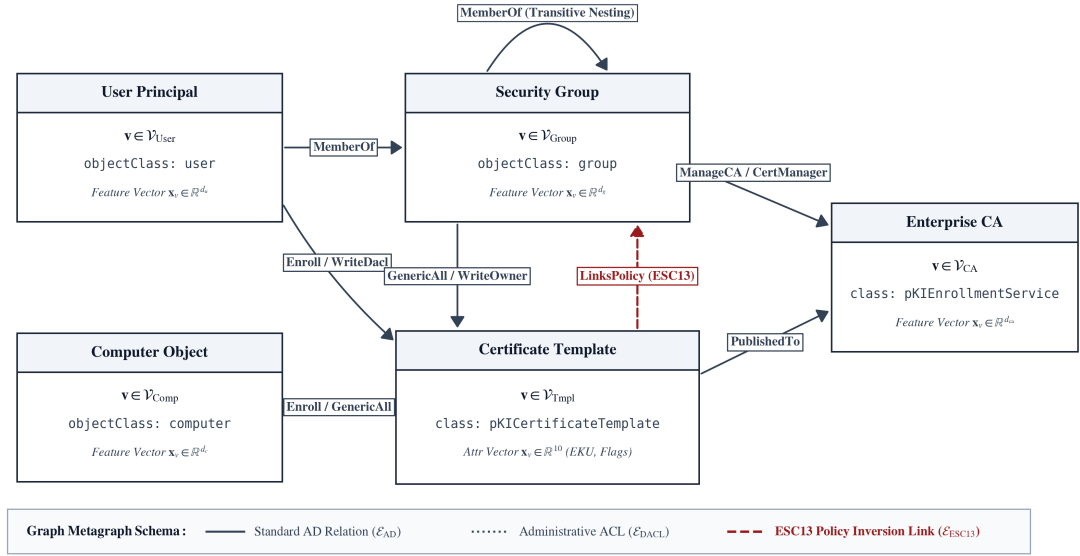
Figure 2.1: Heterogeneous Active Directory Certificate Services (ADCS) Graph Schema, illustrating relations between security principals (Users, Computers, Groups), Certificate Templates, and Enterprise Certificate Authorities.
