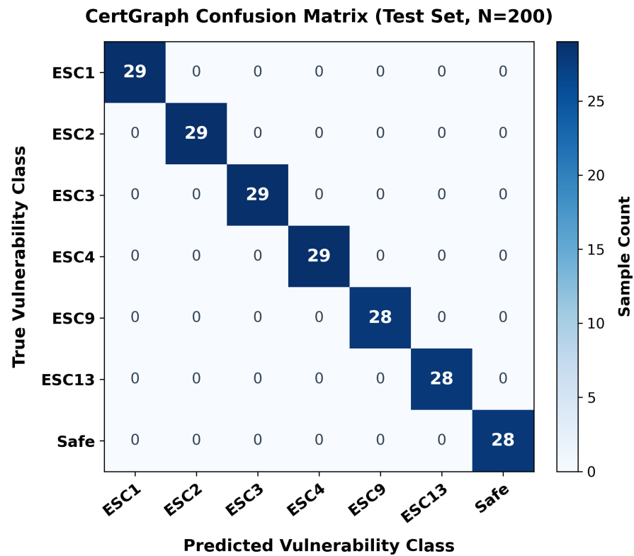
(a) CertGraph 7-Class Confusion Matrix.
