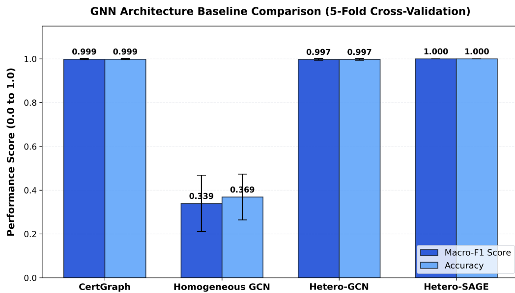
(b) GNN Family Comparison.
