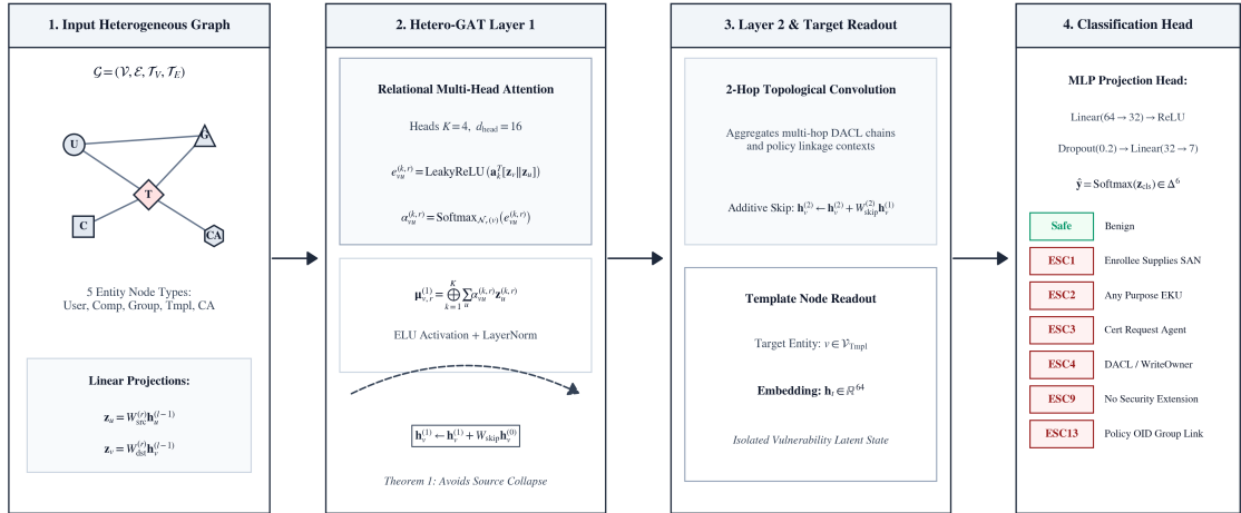
Figure 3.1: CertGraph end-to-end Hetero-GAT pipeline, detailing input feature encoding, multi-head relational attention layers, additive residual skip-connections, and the multi-class template classification head.
