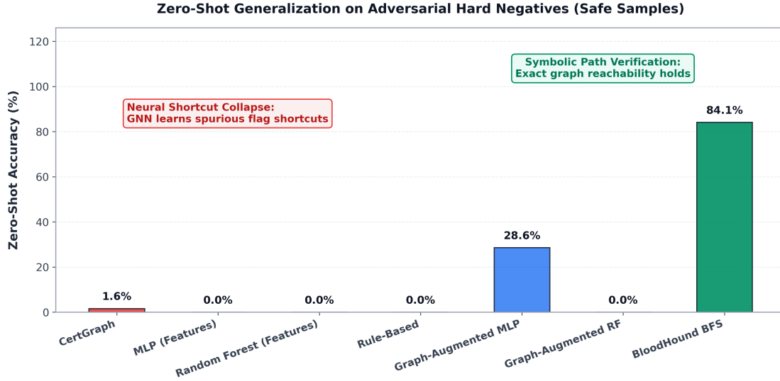
Figure 7: Zero-shot adversarial evaluation demonstrating the collapse of pure neural models due to shortcut learning compared to symbolic BFS path traversal.
