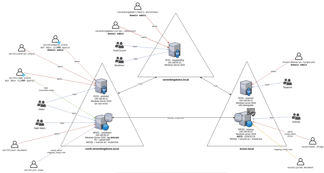
Figure 9: Architecture and trust relationship schema of the Game of Active Directory (GOAD) multi-forest lab environment, detailing domain controllers, member servers (including the ADCS Certificate Authority hosted on SRV03 - braavos ), and cross-forest authentication links.
