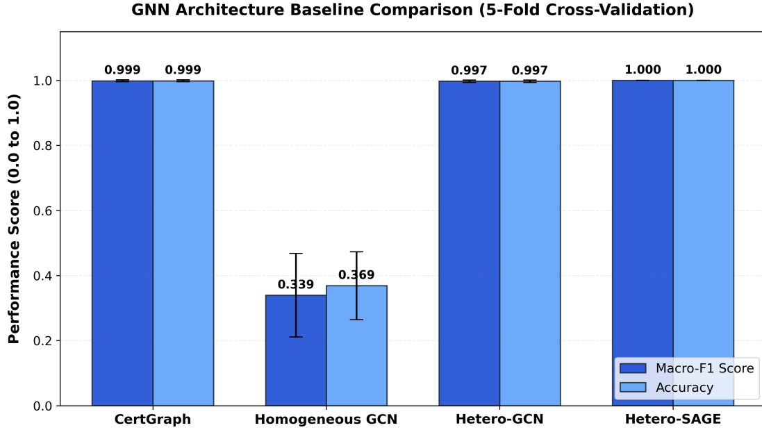
Figure 5: Empirical classification results: (top) Confusion matrix showing near-perfect diagonal alignment across 7 ESC classes; (bottom) Comparison of GNN architectures confirming the empirical superiority of heterogeneous modeling.
