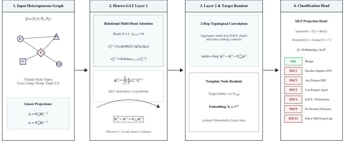
Figure 3: CertGraph end-to-end Hetero-GAT pipeline, detailing input feature encoding, multi-head relational attention layers, additive residual skip-connections, and the multi-class template classification head.
