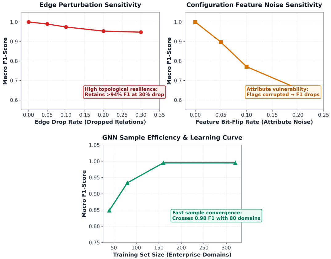
Figure 12: GNN robustness evaluation under systematic edge deletions (collection gaps), configuration feature noise (attribute corruption), and training data efficiency scaling.
