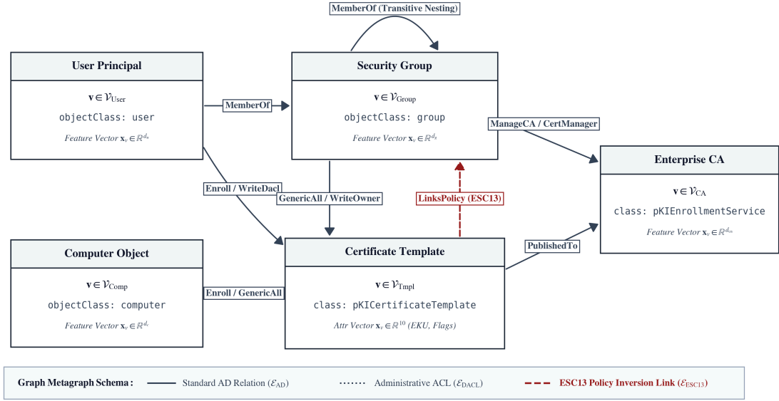
Figure 1: Heterogeneous Active Directory Certificate Services (ADCS) Graph Schema, illustrating relations between security principals (Users, Computers, Groups), Certificate Templates, and Enterprise Certificate Authorities.
