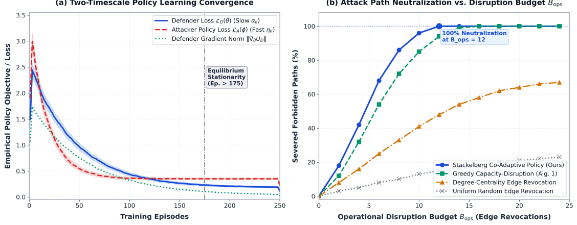
Figure 15: Autonomous cyber defense evaluation: (a) Multi-agent two-timescale policy learning convergence showing the asymptotic decay of defender policy loss and gradient norm over 250 training episodes across 5 independent seeds. (b) Forbidden compromise path neutralization rate as a function of operational disruption budget B_{\text{ops}} , showing that the Stackelberg co-adaptive policy achieves 100% neutralization at B_{\text{ops}} = 12 by identifying high-centrality structural bottlenecks.
