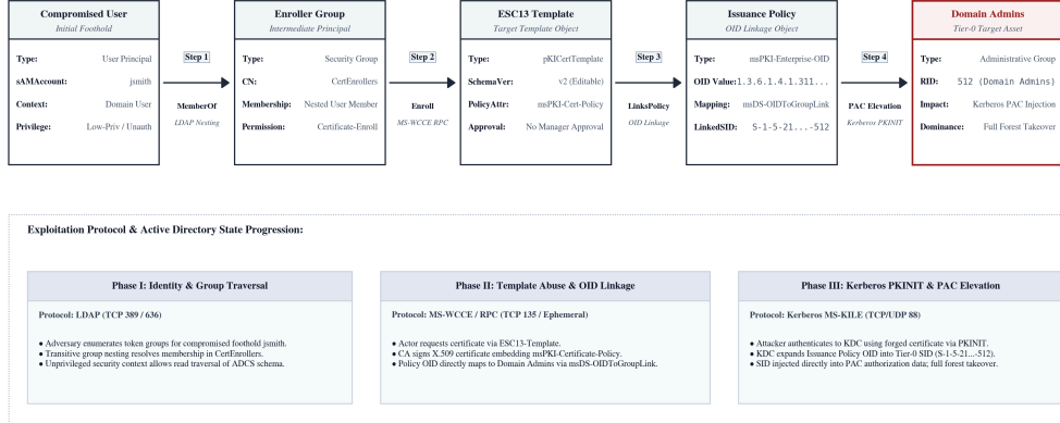
Figure 2: Two-hop ESC13 privilege escalation attack path, showing the chain from an unprivileged user through enrollment permissions and issuance policy OID linkage to high-value domain administrative group tokens.
