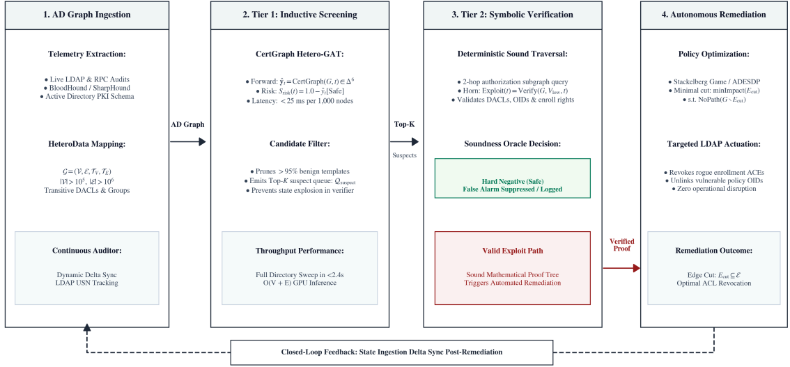
Figure 14: The Two-Tier Neuro-Symbolic Architecture, pairing fast CertGraph GNN screening for risk prioritization with deterministic BloodHound BFS path verification.
