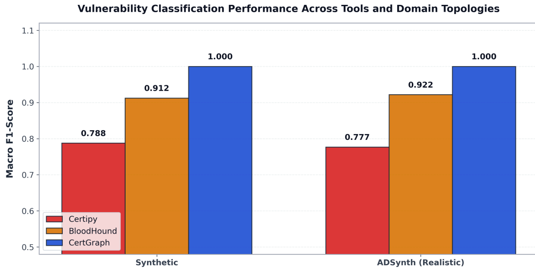
Figure 11: Comparative performance (CertGraph vs BloodHound vs Certipy) across synthetic and ADSynth realistic tiered enterprise topologies.
