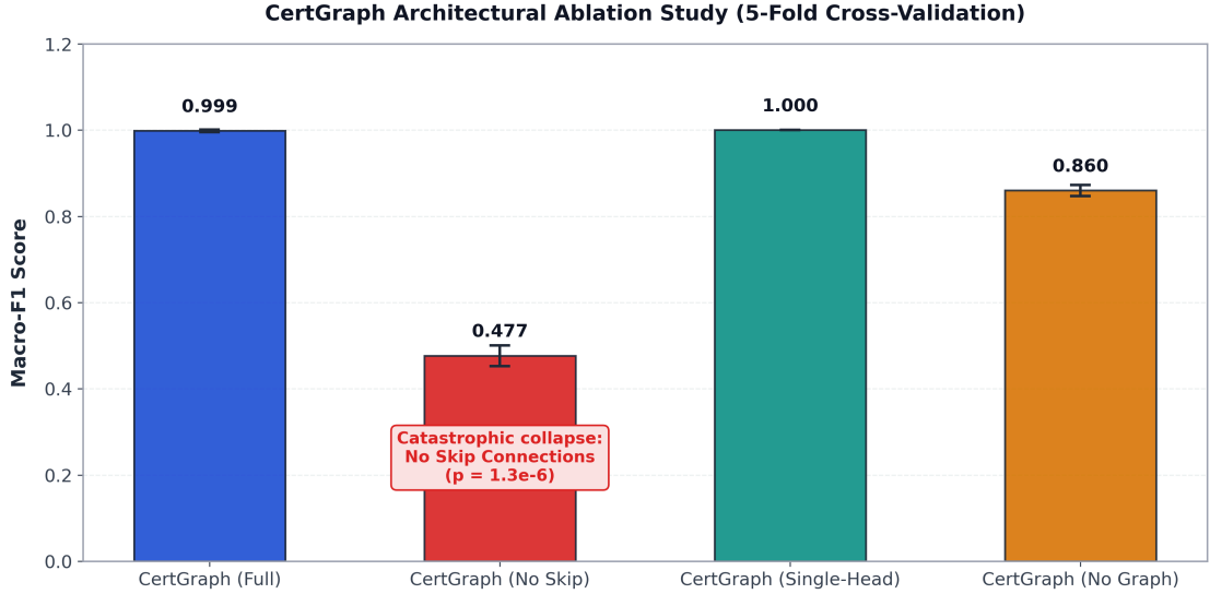
Figure 6: Ablation study comparison highlighting the performance collapse when residual skip connections are disabled.
