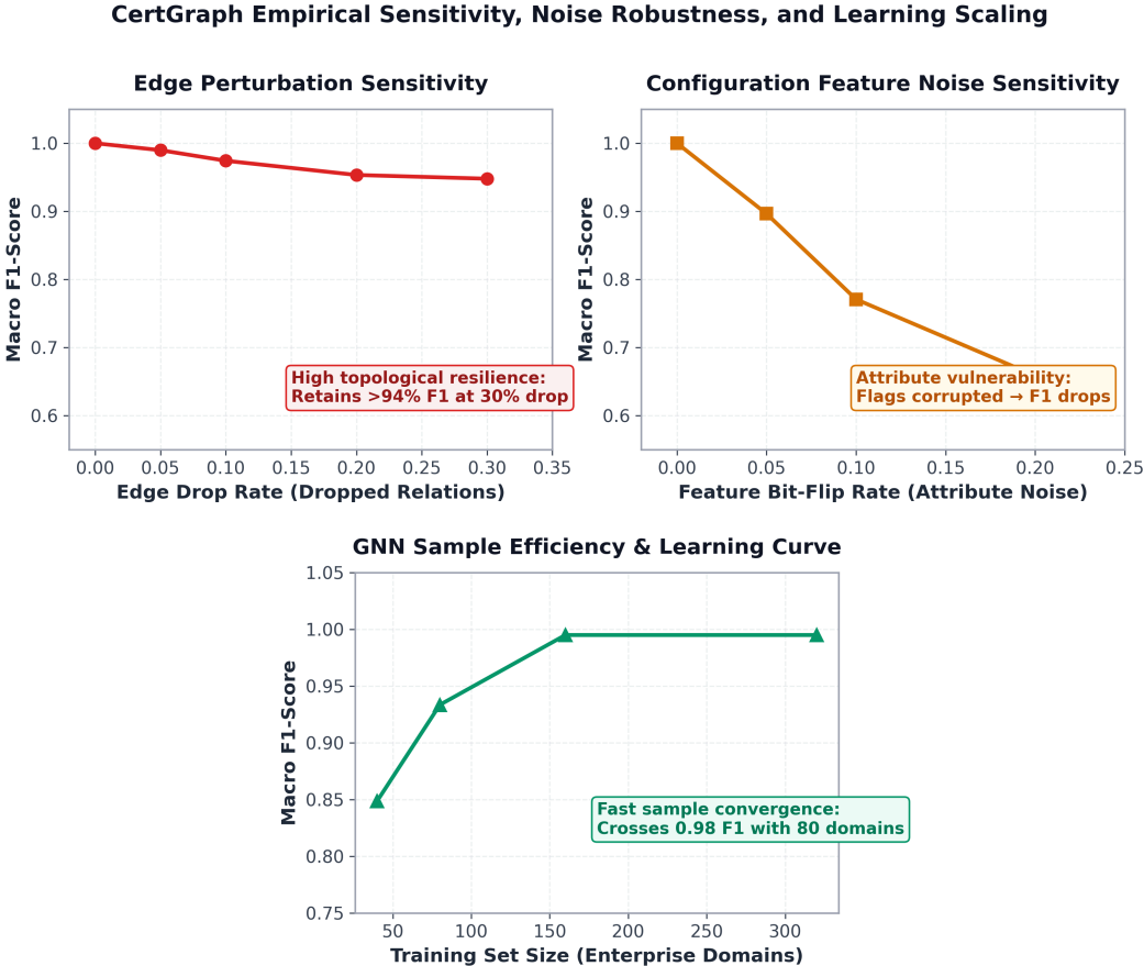
Figure 12: GNN robustness evaluation under systematic edge deletions (collection gaps), configuration feature noise (attribute corruption), and training data efficiency scaling.
