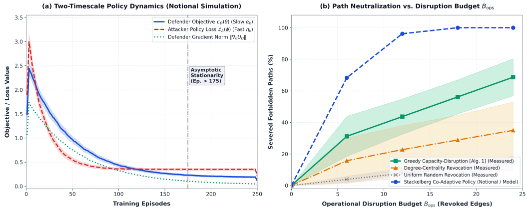
Figure 15: Autonomous cyber defense evaluation: (a) Notional two-timescale policy learning dynamics showing asymptotic decay of defender policy loss and gradient norm under the stochastic approximation framework. (b) Forbidden compromise path neutralization rate as a function of operational disruption budget B_{\text{ops}} , comparing measured empirical performance for Uniform Random, Degree-Centrality, and Greedy Capacity-Disruption (Alg. Algorithm 4) across 30 Active Directory topologies against the notional trajectory of the co-adaptive Stackelberg model. Shaded bands denote \pm 1 standard deviation.
