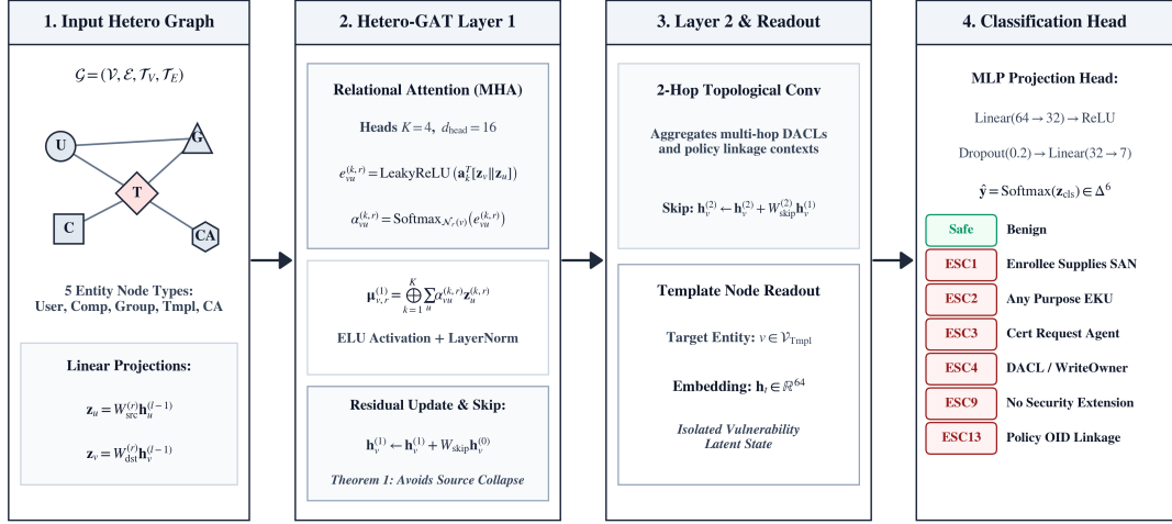
Figure 3.1: CertGraph end-to-end Hetero-GAT pipeline, detailing input feature encoding, multi-head relational attention layers, additive residual skip-connections, and the multi-class template classification head.
