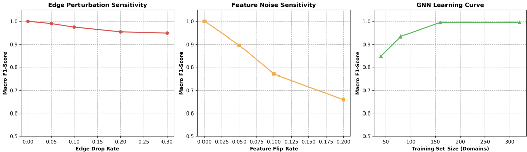
Figure 12: GNN robustness evaluation under systematic edge deletions (collection gaps), configuration feature noise (attribute corruption), and training data efficiency scaling.
