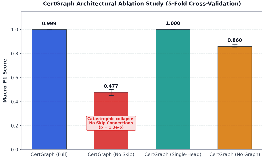
Figure 6: Ablation study comparison highlighting the catastrophic performance collapse when residual skip connections are disabled.
