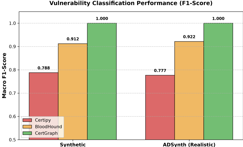
Figure 11: Comparative performance (CertGraph vs BloodHound vs Certipy) across synthetic and ADSynth realistic tiered enterprise topologies.
