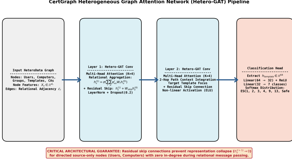
Figure 3: CertGraph end-to-end Hetero-GAT pipeline, detailing input feature encoding, multi-head relational attention layers, additive residual skip-connections, and the multi-class template classification head.
