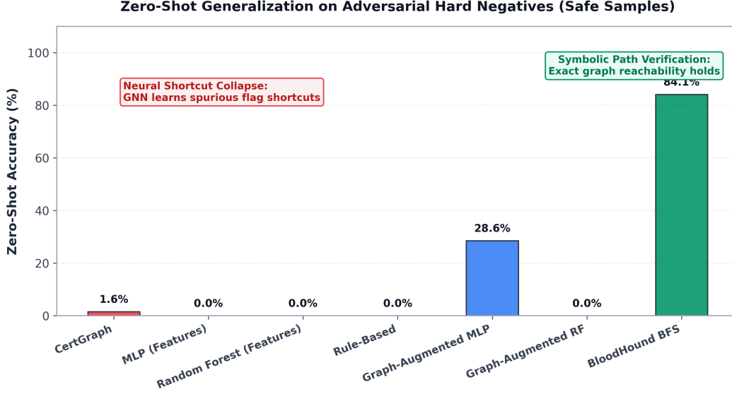
Figure 7: Zero-shot adversarial evaluation demonstrating the catastrophic collapse of neural models due to shortcut learning compared to symbolic BFS path traversal.
