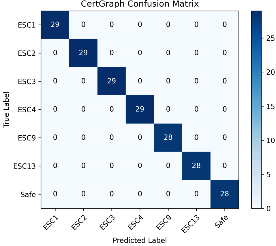
Figure 5: CertGraph 7-Class Confusion Matrix.
