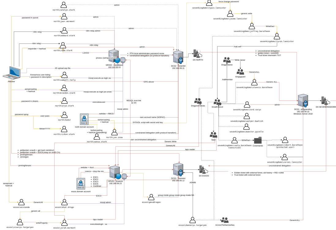
Figure 6.2: End-to-end multi-hop compromise and privilege escalation attack graph across the GOAD domain infrastructure, illustrating how unprivileged foothold credentials traverse AD CS certificate misconfigurations (ESC1–ESC8), Kerberos delegations, and inter-domain trusts to achieve enterprise domain dominance.
