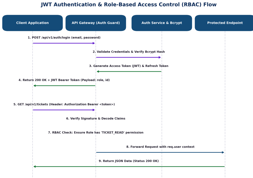
Figure 11: JWT Authentication and Role-Based Access Control (RBAC) Flow.
