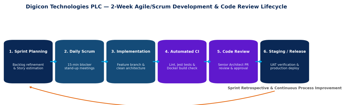
Figure 2: Digicon Agile/Scrum Sprint and Code Review Lifecycle.
