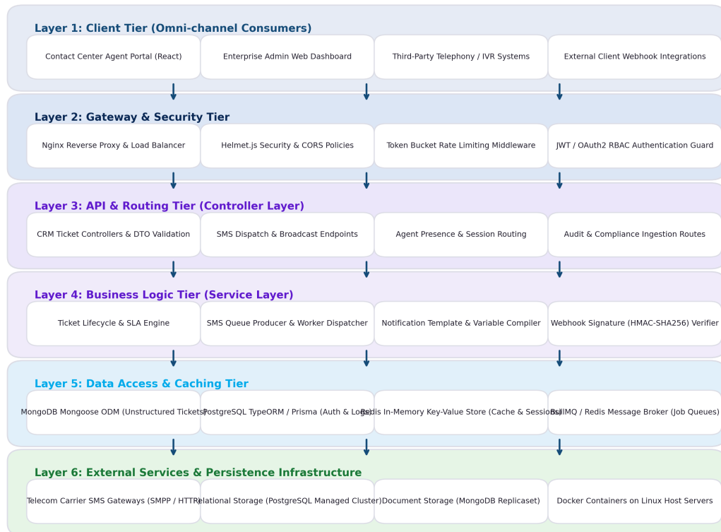
Figure 5: Digicon Backend System — Layered Microservices Architecture.
