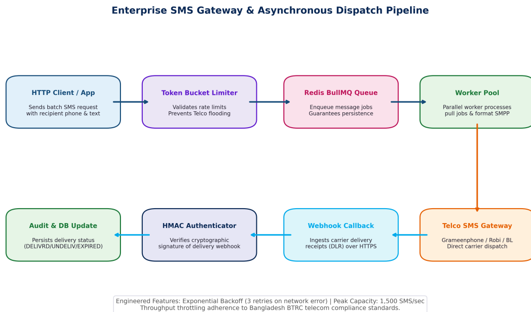
Figure 9: Enterprise SMS Gateway and Asynchronous Dispatch Pipeline.
