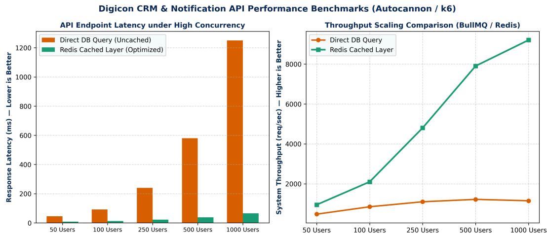
Figure 16: Digicon CRM API Performance Benchmarks under Increasing Concurrency (Autocannon / k6).
