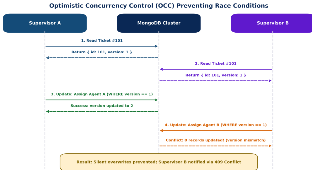
Figure 13: Optimistic Concurrency Control Sequence in Ticket Assignment.
