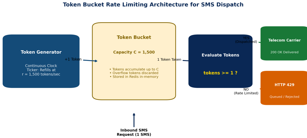
Figure 10: Token Bucket Rate Limiting Algorithm Execution Flow.
