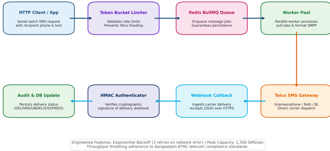
Figure 6: Enterprise SMS Gateway and Asynchronous Dispatch Pipeline.
