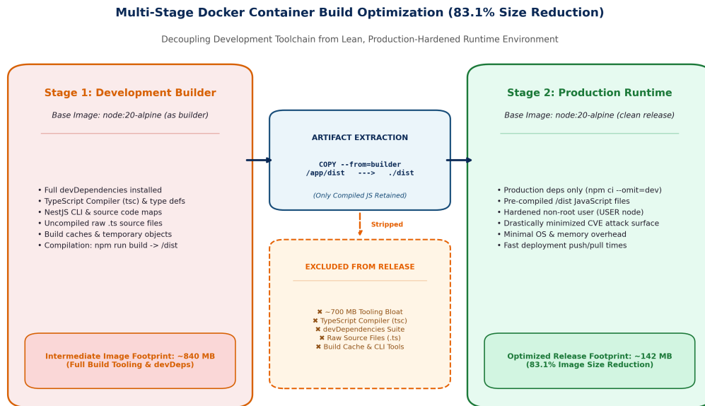
Figure 17: Multi-Stage Docker Build Architecture and Image Size Optimization.
